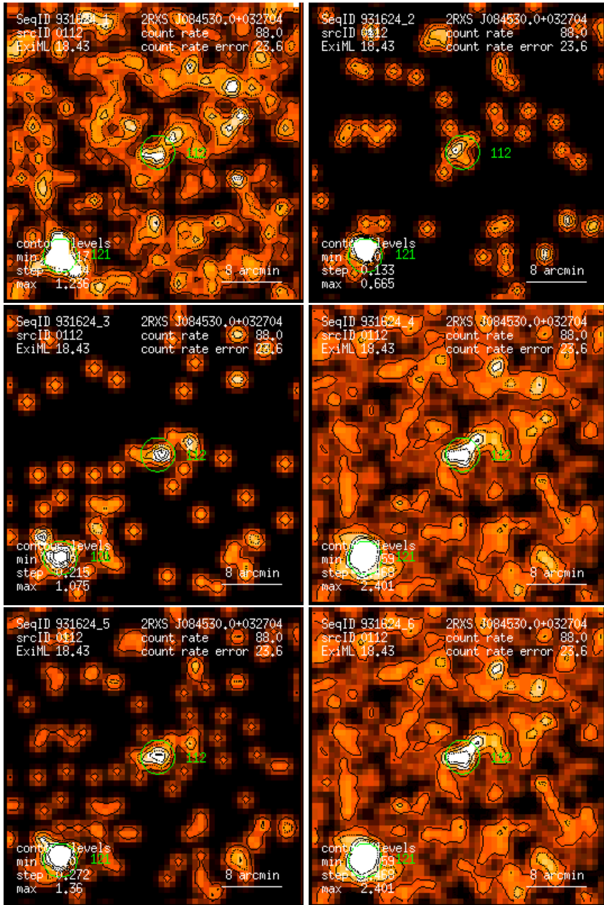
Figure 112: RASS 931624: detection 0112: band rate images, Gaussian filter: (1) PSPC channels 11 – 41, (2) 52 – 90, (3) 91 – 201, (4) 11 – 235, (5) 52 – 201, (6) 11 – 201. Broad band rates in counts/ks. Band rate contour levels in counts/ks/arcmin 2 .
