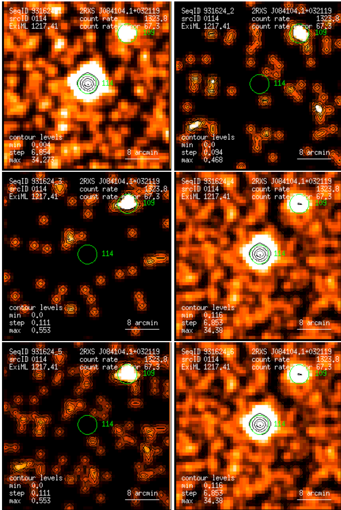
Figure 114: RASS 931624: detection 0114: band rate images, Gaussian filter: (1) PSPC channels 11 – 41, (2) 52 – 90, (3) 91 – 201, (4) 11 – 235, (5) 52 – 201, (6) 11 – 201. Broad band rates in counts/ks. Band rate contour levels in counts/ks/arcmin 2 .
