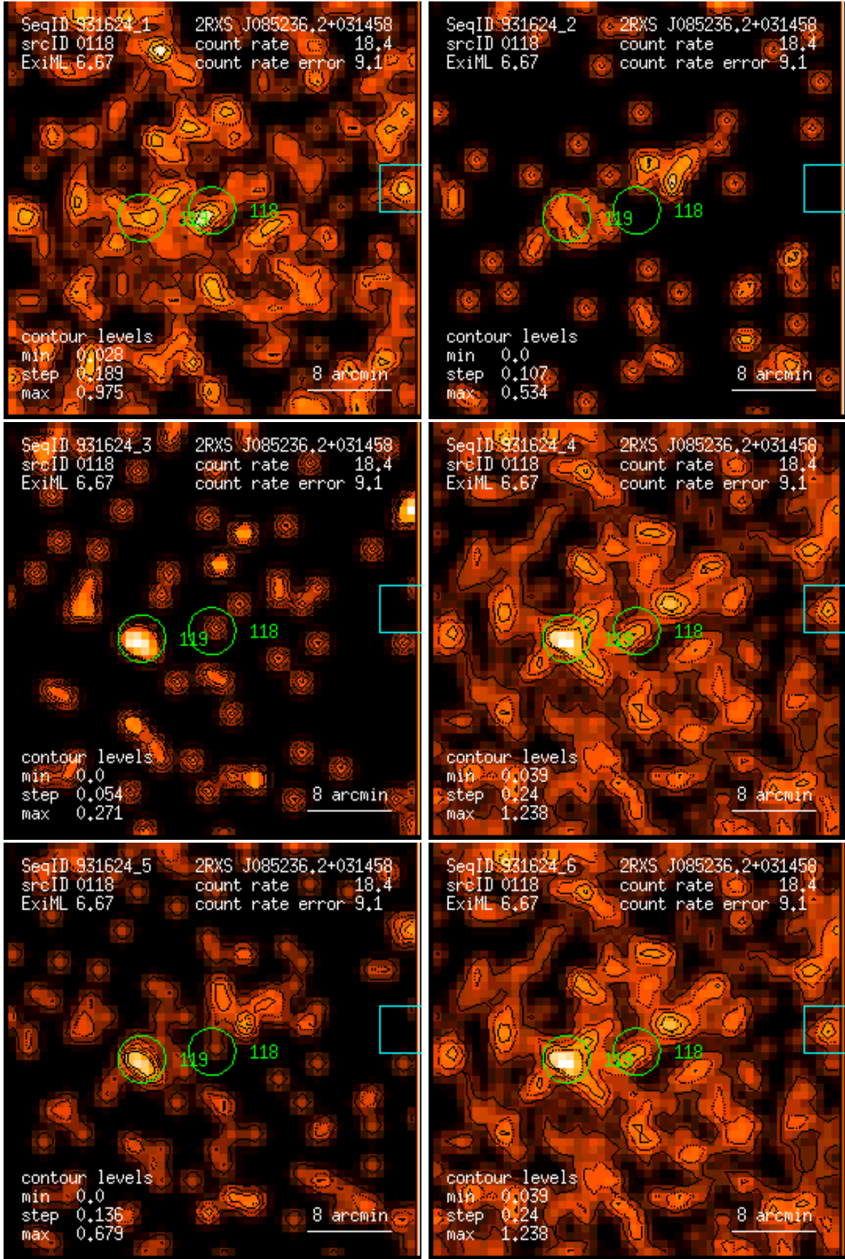
Figure 118: RASS 931624: detection 0118: band rate images, Gaussian filter: (1) PSPC channels 11 – 41, (2) 52 – 90, (3) 91 – 201, (4) 11 – 235, (5) 52 – 201, (6) 11 – 201. Broad band rates in counts/ks. Band rate contour levels in counts/ks/arcmin 2 .
