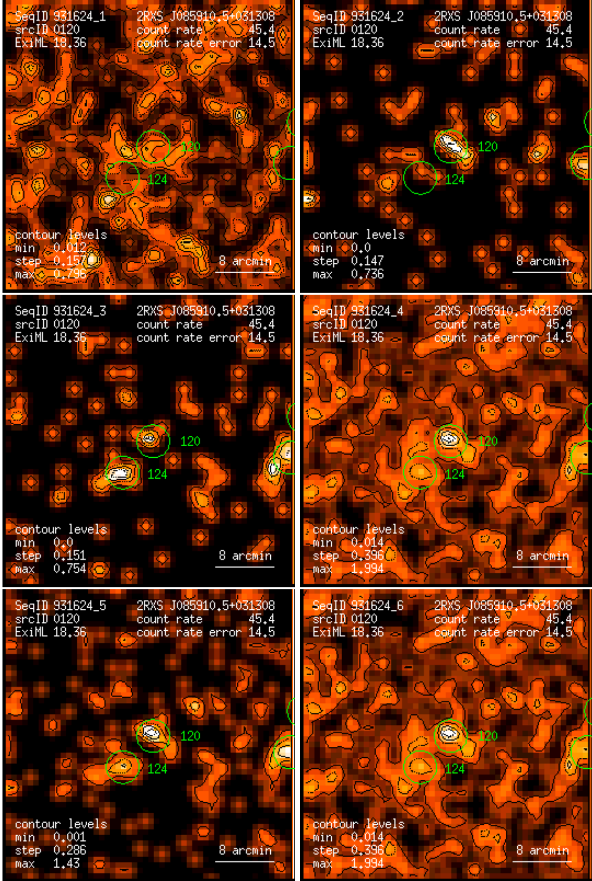
Figure 120: RASS 931624: detection 0120: band rate images, Gaussian filter: (1) PSPC channels 11 – 41, (2) 52 – 90, (3) 91 – 201, (4) 11 – 235, (5) 52 – 201, (6) 11 – 201. Broad band rates in counts/ks. Band rate contour levels in counts/ks/arcmin 2 .
