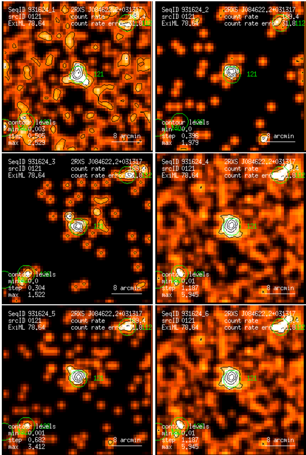
Figure 121: RASS 931624: detection 0121: band rate images, Gaussian filter: (1) PSPC channels 11 – 41, (2) 52 – 90, (3) 91 – 201, (4) 11 – 235, (5) 52 – 201, (6) 11 – 201. Broad band rates in counts/ks. Band rate contour levels in counts/ks/arcmin 2 .
