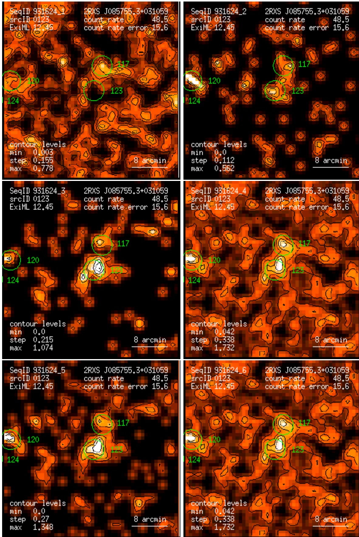
Figure 123: RASS 931624: detection 0123: band rate images, Gaussian filter: (1) PSPC channels 11 – 41, (2) 52 – 90, (3) 91 – 201, (4) 11 – 235, (5) 52 – 201, (6) 11 – 201. Broad band rates in counts/ks. Band rate contour levels in counts/ks/arcmin 2 .
