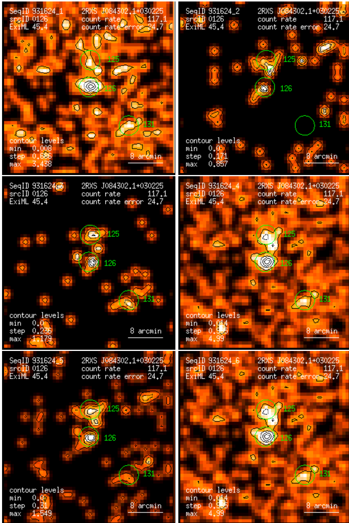
Figure 126: RASS 931624: detection 0126: band rate images, Gaussian filter: (1) PSPC channels 11 – 41, (2) 52 – 90, (3) 91 – 201, (4) 11 – 235, (5) 52 – 201, (6) 11 – 201. Broad band rates in counts/ks. Band rate contour levels in counts/ks/arcmin 2 .
