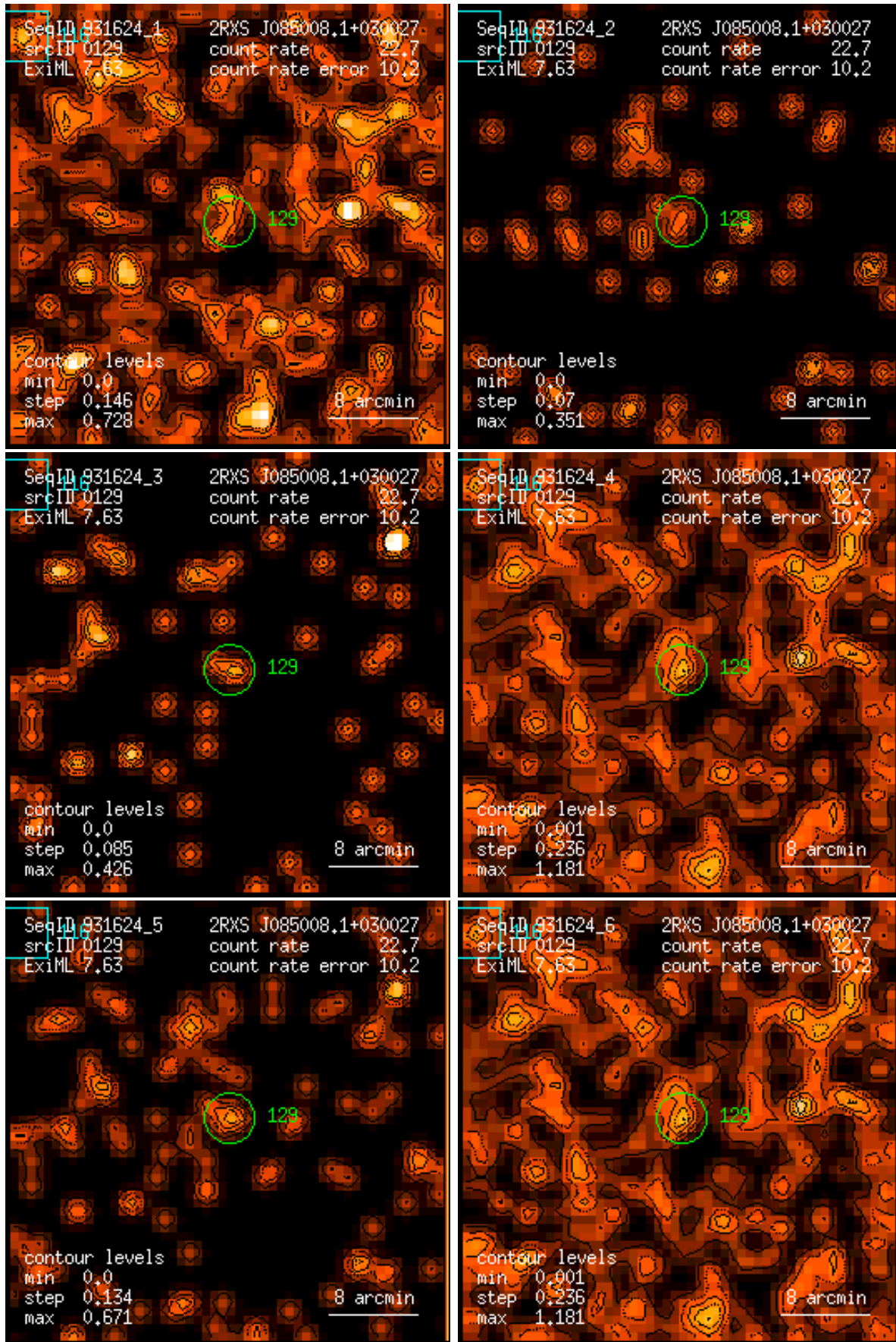
Figure 129: RASS 931624: detection 0129: band rate images, Gaussian filter: (1) PSPC channels 11 – 41, (2) 52 – 90, (3) 91 – 201, (4) 11 – 235, (5) 52 – 201, (6) 11 – 201. Broad band rates in counts/ks. Band rate contour levels in counts/ks/arcmin 2 .
