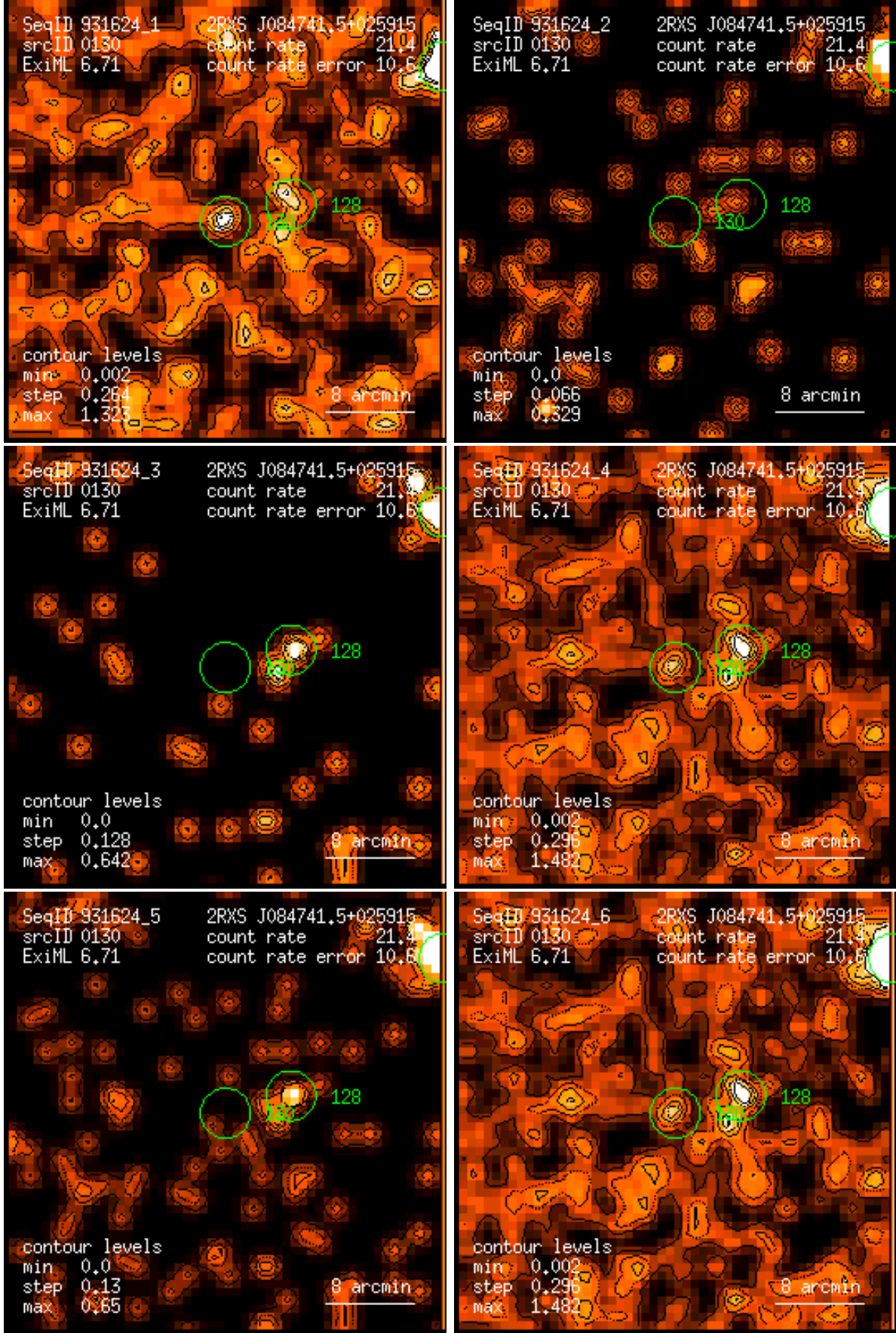
Figure 130: RASS 931624: detection 0130: band rate images, Gaussian filter: (1) PSPC channels 11 – 41, (2) 52 – 90, (3) 91 – 201, (4) 11 – 235, (5) 52 – 201, (6) 11 – 201. Broad band rates in counts/ks. Band rate contour levels in counts/ks/arcmin 2 .
