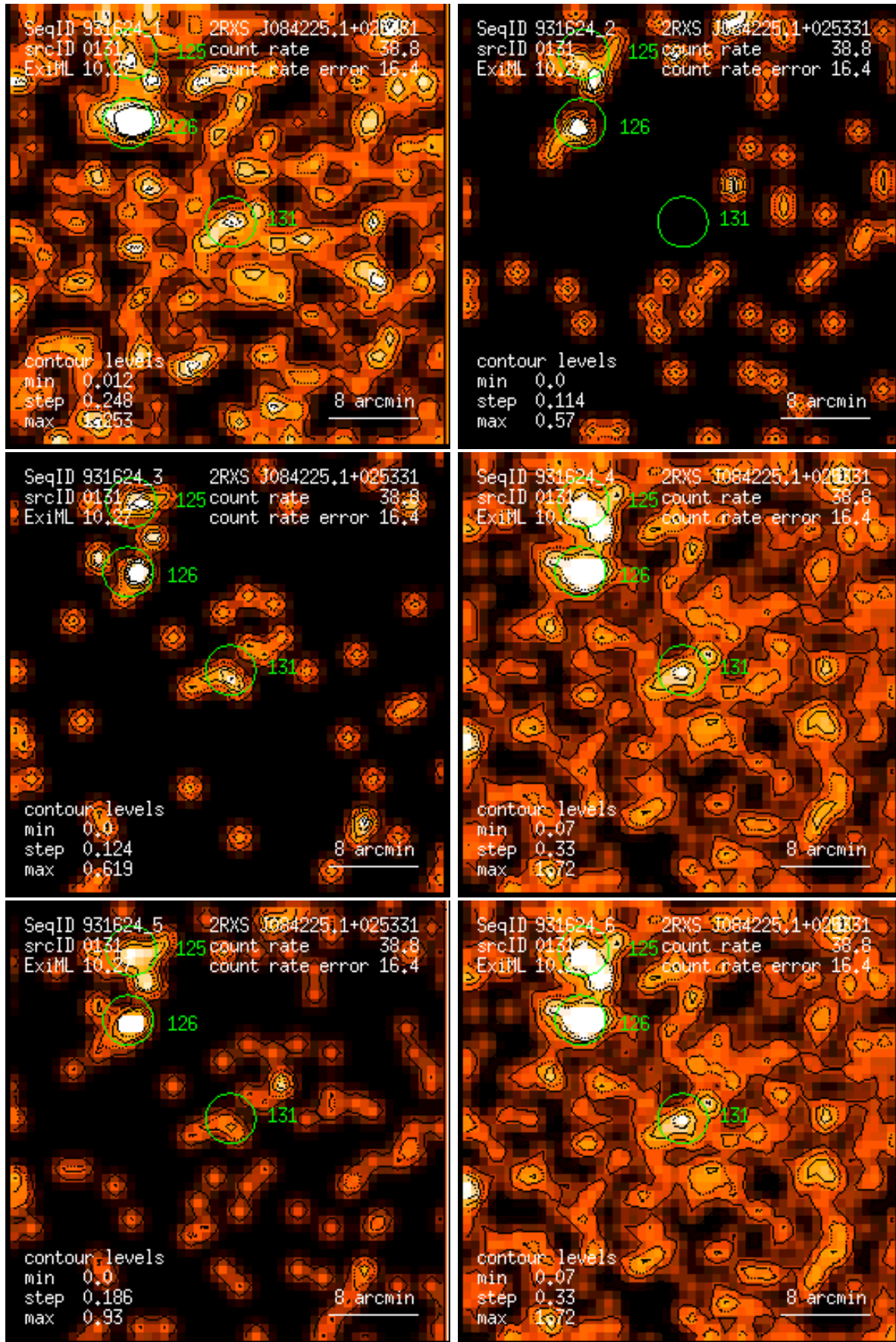
Figure 131: RASS 931624: detection 0131: band rate images, Gaussian filter: (1) PSPC channels 11 – 41, (2) 52 – 90, (3) 91 – 201, (4) 11 – 235, (5) 52 – 201, (6) 11 – 201. Broad band rates in counts/ks. Band rate contour levels in counts/ks/arcmin 2 .
