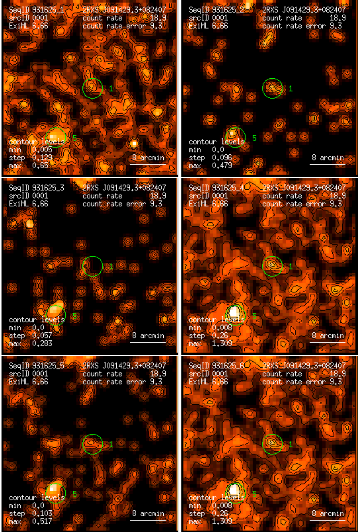
Figure 1: RASS 931625: detection 0001: band rate images, Gaussian filter: (1) PSPC channels 11 – 41, (2) 52 – 90, (3) 91 – 201, (4) 11 – 235, (5) 52 – 201, (6) 11 – 201. Broad band rates in counts/ks. Band rate contour levels in counts/ks/arcmin 2 .
