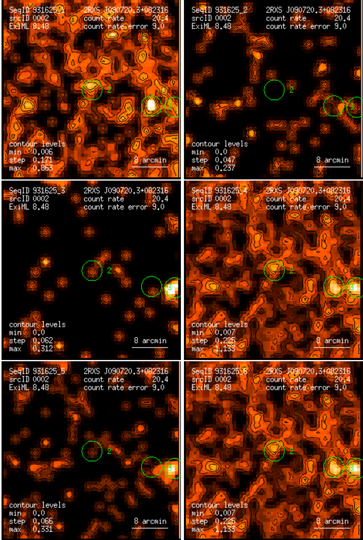
Figure 2: RASS 931625: detection 0002: band rate images, Gaussian filter: (1) PSPC channels 11 – 41, (2) 52 – 90, (3) 91 – 201, (4) 11 – 235, (5) 52 – 201, (6) 11 – 201. Broad band rates in counts/ks. Band rate contour levels in counts/ks/arcmin 2 .
