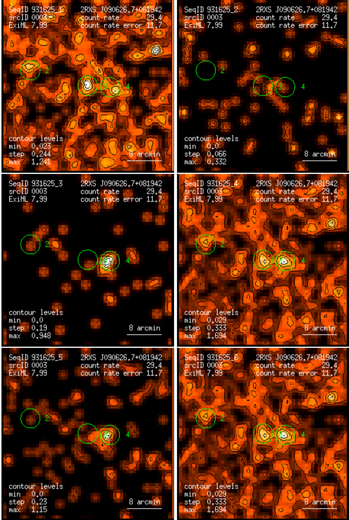
Figure 3: RASS 931625: detection 0003: band rate images, Gaussian filter: (1) PSPC channels 11 – 41, (2) 52 – 90, (3) 91 – 201, (4) 11 – 235, (5) 52 – 201, (6) 11 – 201. Broad band rates in counts/ks. Band rate contour levels in counts/ks/arcmin 2 .
