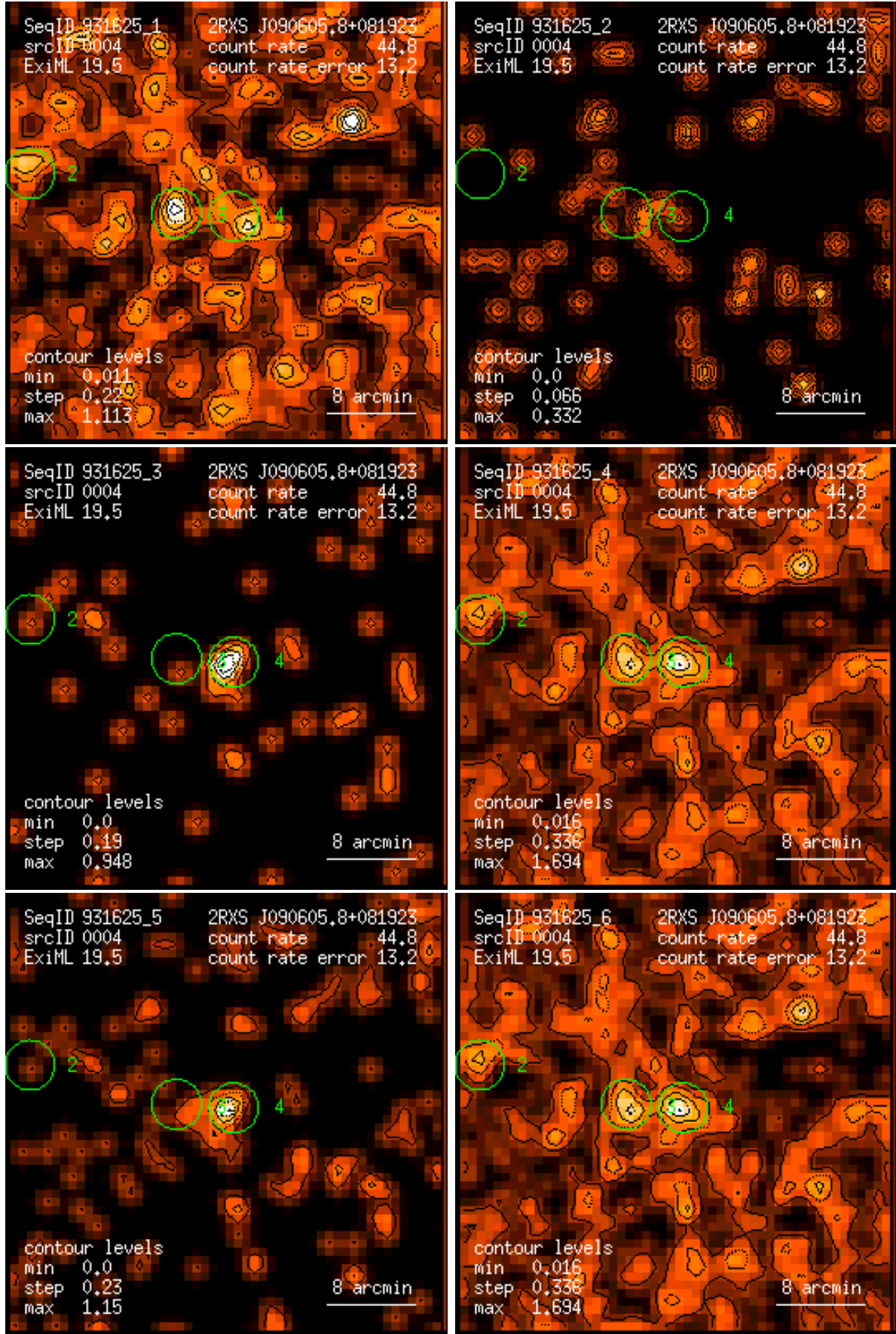
Figure 4: RASS 931625: detection 0004: band rate images, Gaussian filter: (1) PSPC channels 11 – 41, (2) 52 – 90, (3) 91 – 201, (4) 11 – 235, (5) 52 – 201, (6) 11 – 201. Broad band rates in counts/ks. Band rate contour levels in counts/ks/arcmin 2 .
