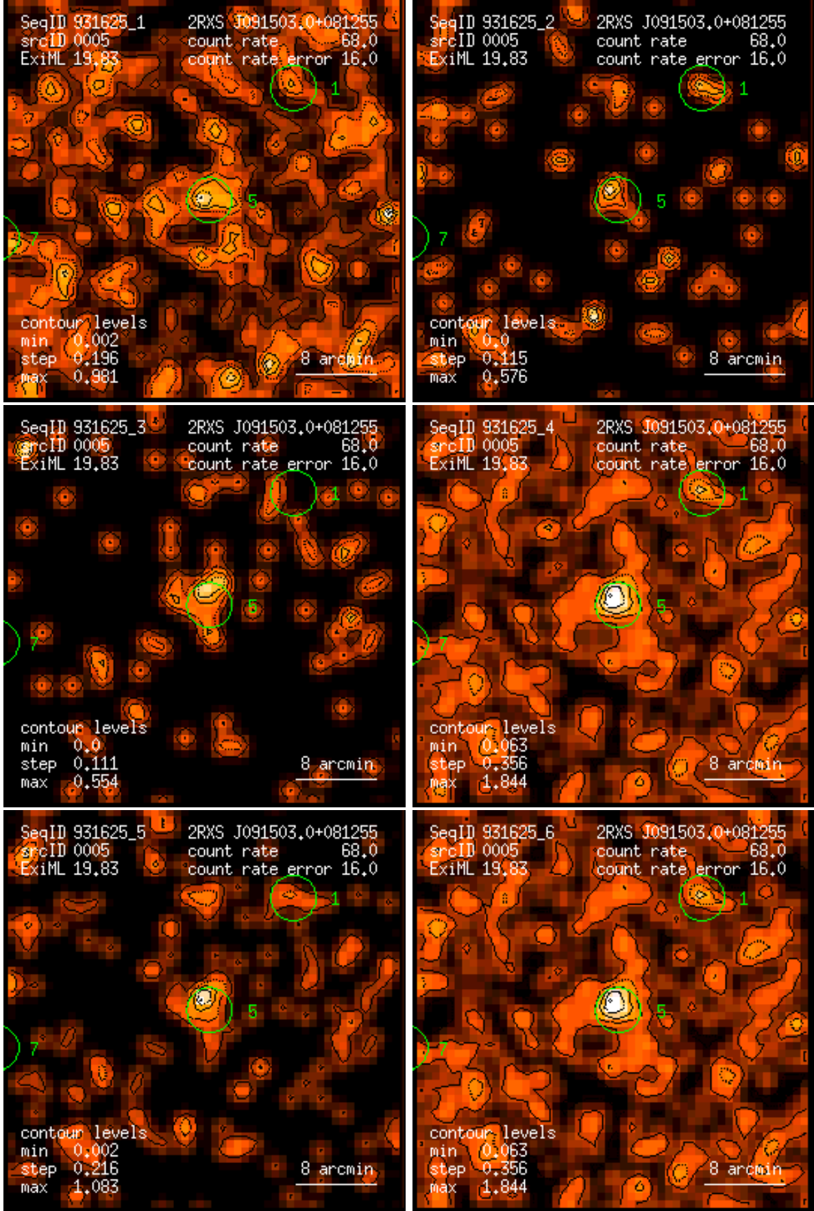
Figure 5: RASS 931625: detection 0005: band rate images, Gaussian filter: (1) PSPC channels 11 – 41, (2) 52 – 90, (3) 91 – 201, (4) 11 – 235, (5) 52 – 201, (6) 11 – 201. Broad band rates in counts/ks. Band rate contour levels in counts/ks/arcmin 2 .
