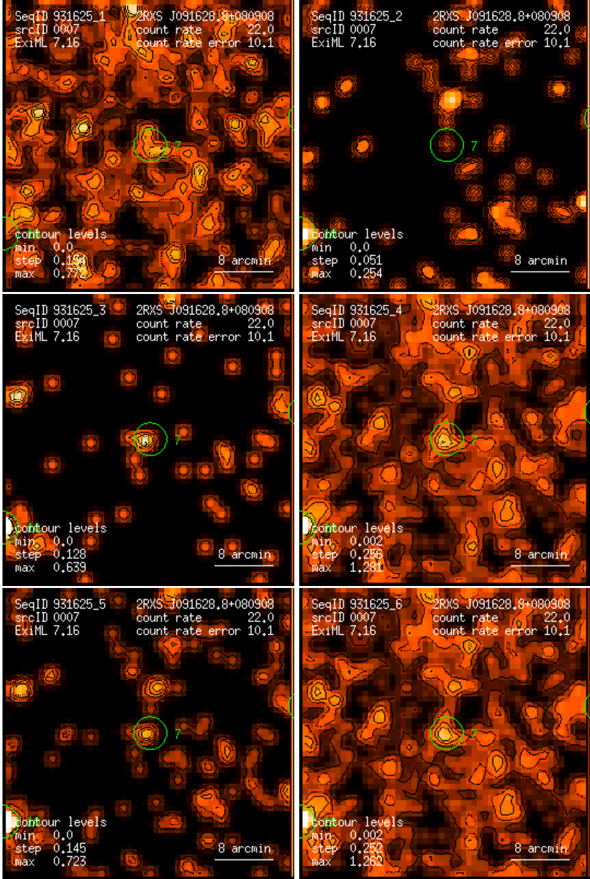
Figure 7: RASS 931625: detection 0007: band rate images, Gaussian filter: (1) PSPC channels 11 – 41, (2) 52 – 90, (3) 91 – 201, (4) 11 – 235, (5) 52 – 201, (6) 11 – 201. Broad band rates in counts/ks. Band rate contour levels in counts/ks/arcmin 2 .
