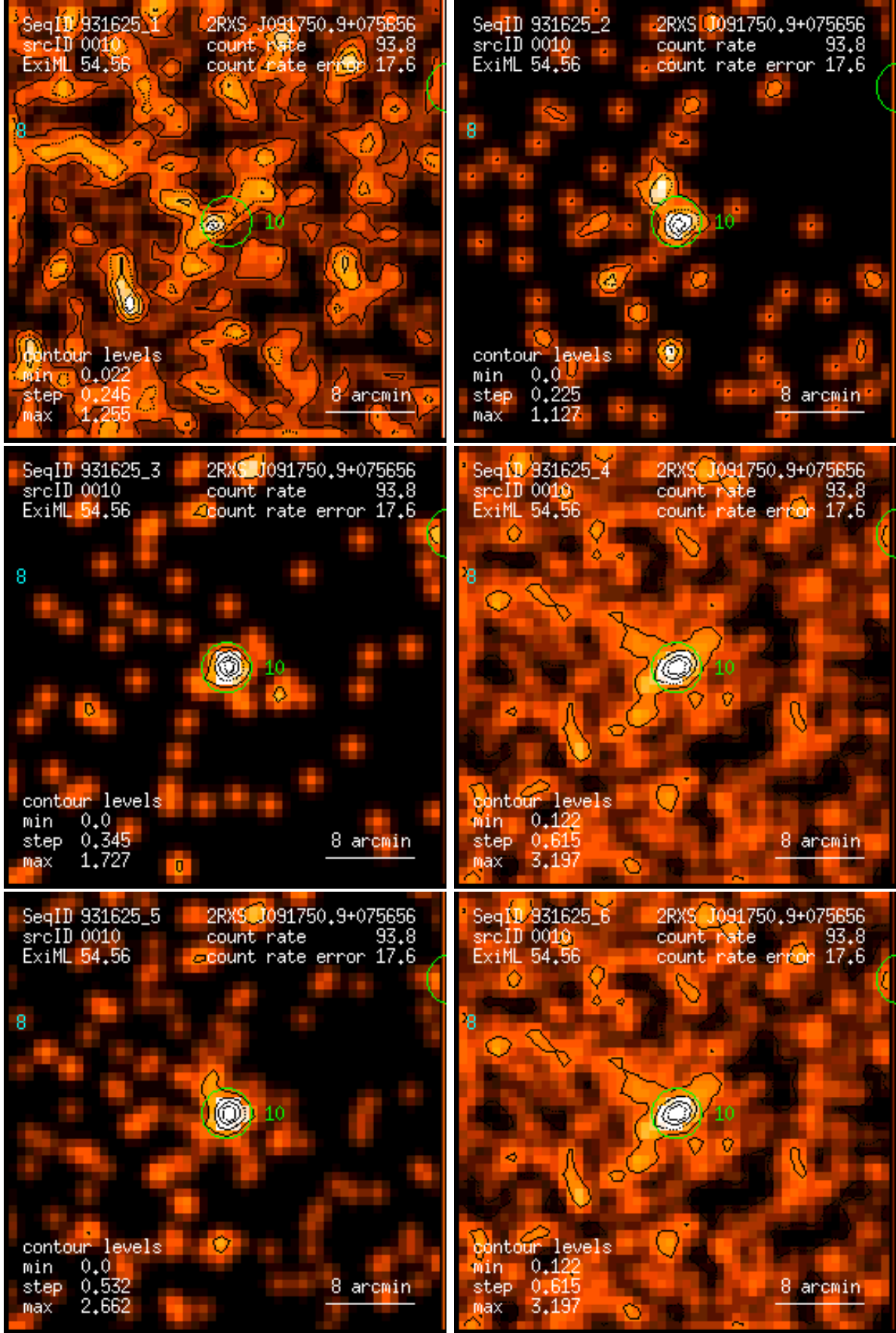
Figure 10: RASS 931625: detection 0010: band rate images, Gaussian filter: (1) PSPC channels 11 – 41, (2) 52 – 90, (3) 91 – 201, (4) 11 – 235, (5) 52 – 201, (6) 11 – 201. Broad band rates in counts/ks. Band rate contour levels in counts/ks/arcmin 2 .
