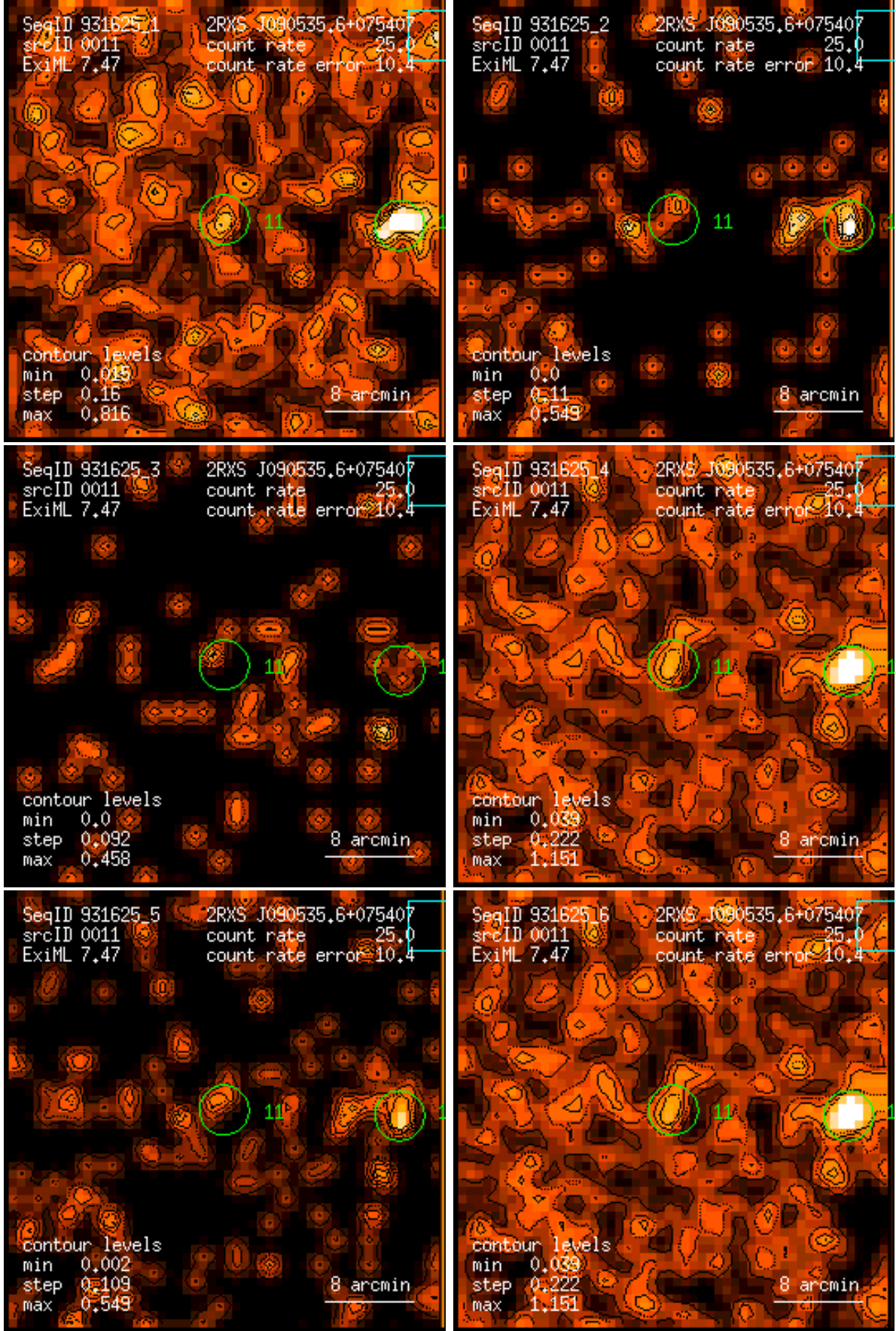
Figure 11: RASS 931625: detection 0011: band rate images, Gaussian filter: (1) PSPC channels 11 – 41, (2) 52 – 90, (3) 91 – 201, (4) 11 – 235, (5) 52 – 201, (6) 11 – 201. Broad band rates in counts/ks. Band rate contour levels in counts/ks/arcmin 2 .
