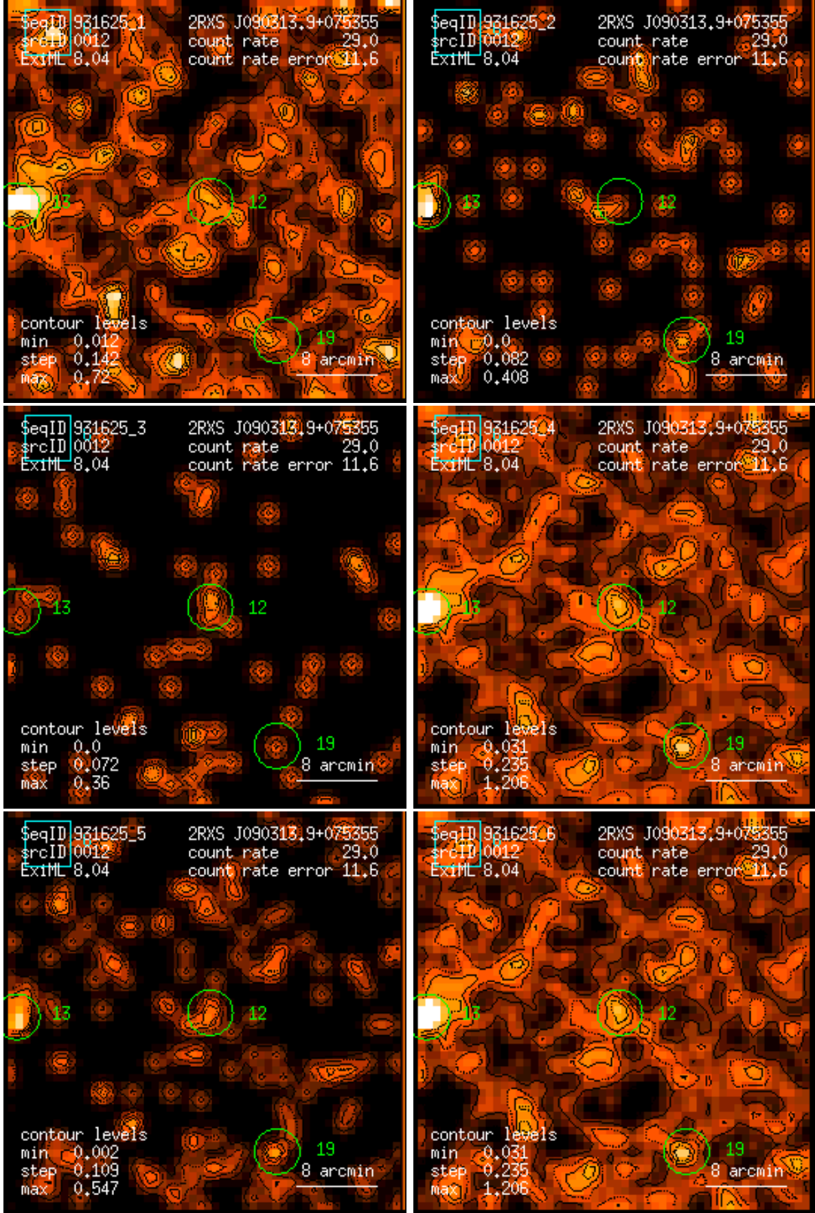
Figure 12: RASS 931625: detection 0012: band rate images, Gaussian filter: (1) PSPC channels 11 – 41, (2) 52 – 90, (3) 91 – 201, (4) 11 – 235, (5) 52 – 201, (6) 11 – 201. Broad band rates in counts/ks. Band rate contour levels in counts/ks/arcmin 2 .
