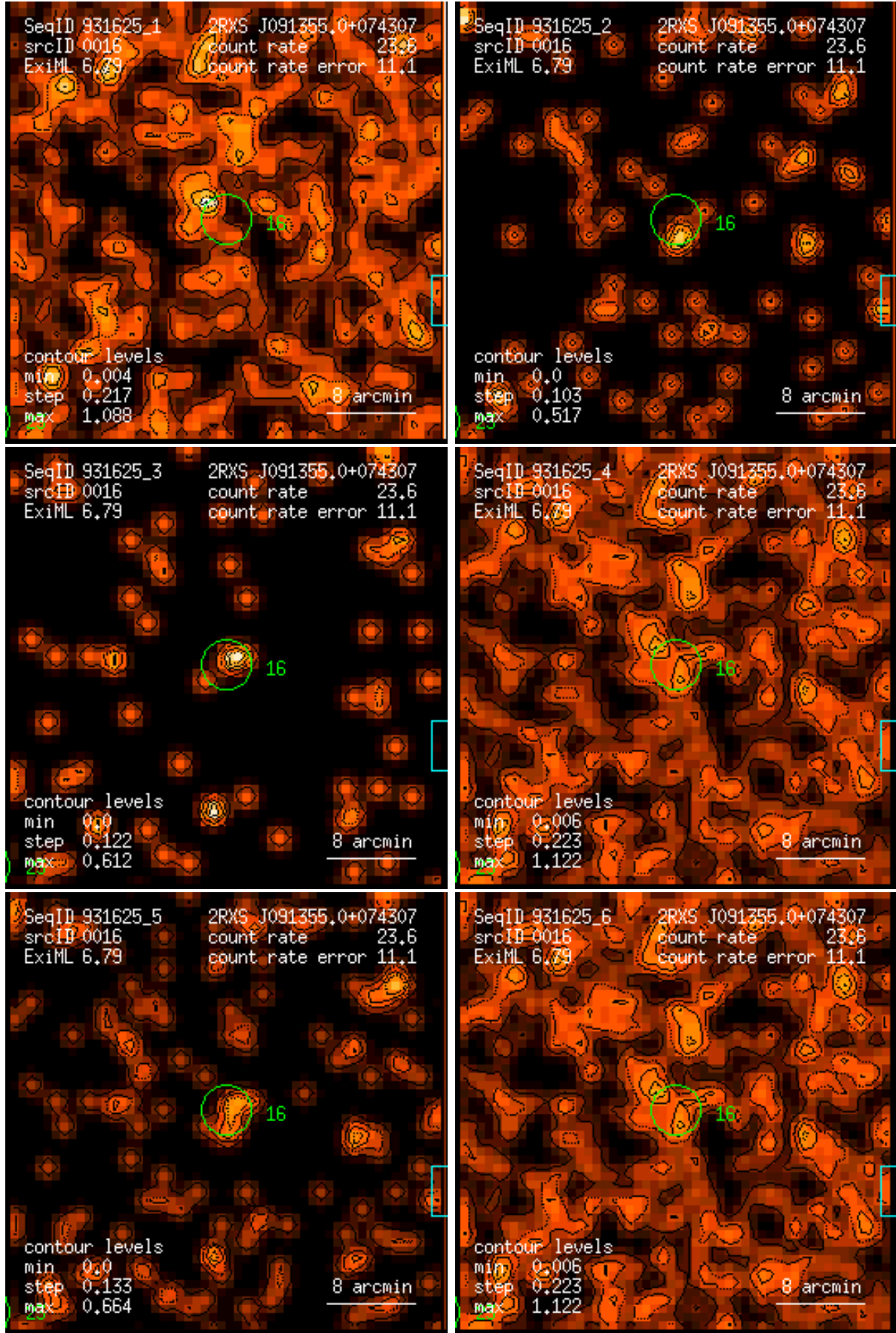
Figure 16: RASS 931625: detection 0016: band rate images, Gaussian filter: (1) PSPC channels 11 – 41, (2) 52 – 90, (3) 91 – 201, (4) 11 – 235, (5) 52 – 201, (6) 11 – 201. Broad band rates in counts/ks. Band rate contour levels in counts/ks/arcmin 2 .
