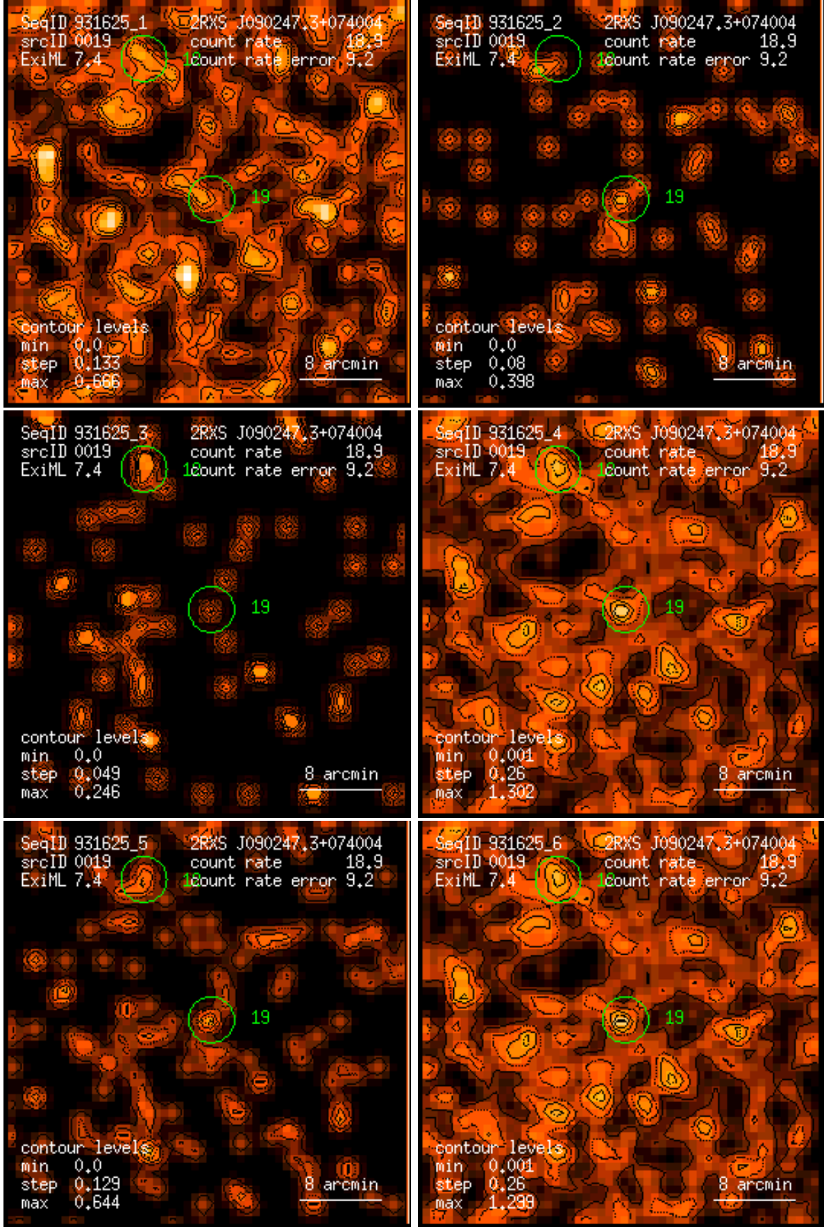
Figure 19: RASS 931625: detection 0019: band rate images, Gaussian filter: (1) PSPC channels 11 – 41, (2) 52 – 90, (3) 91 – 201, (4) 11 – 235, (5) 52 – 201, (6) 11 – 201. Broad band rates in counts/ks. Band rate contour levels in counts/ks/arcmin 2 .
