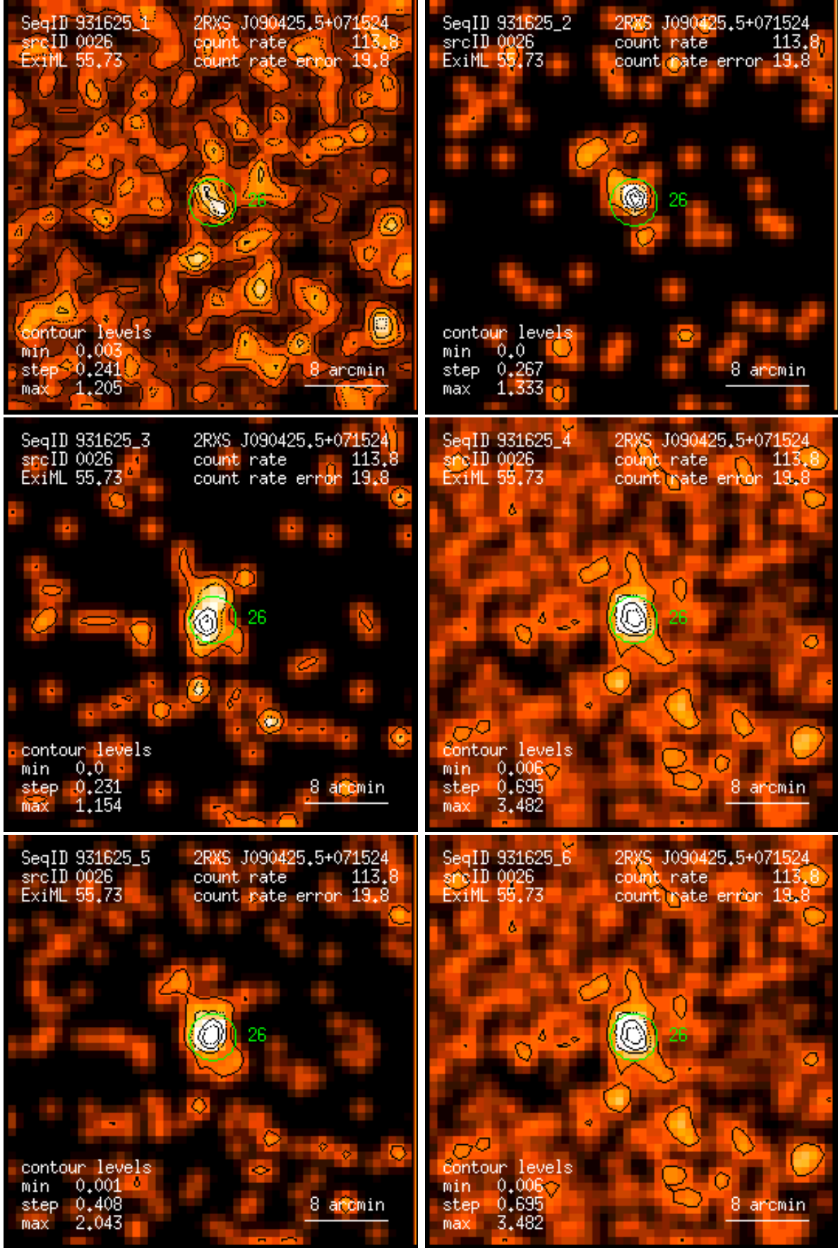
Figure 26: RASS 931625: detection 0026: band rate images, Gaussian filter: (1) PSPC channels 11 – 41, (2) 52 – 90, (3) 91 – 201, (4) 11 – 235, (5) 52 – 201, (6) 11 – 201. Broad band rates in counts/ks. Band rate contour levels in counts/ks/arcmin 2 .
