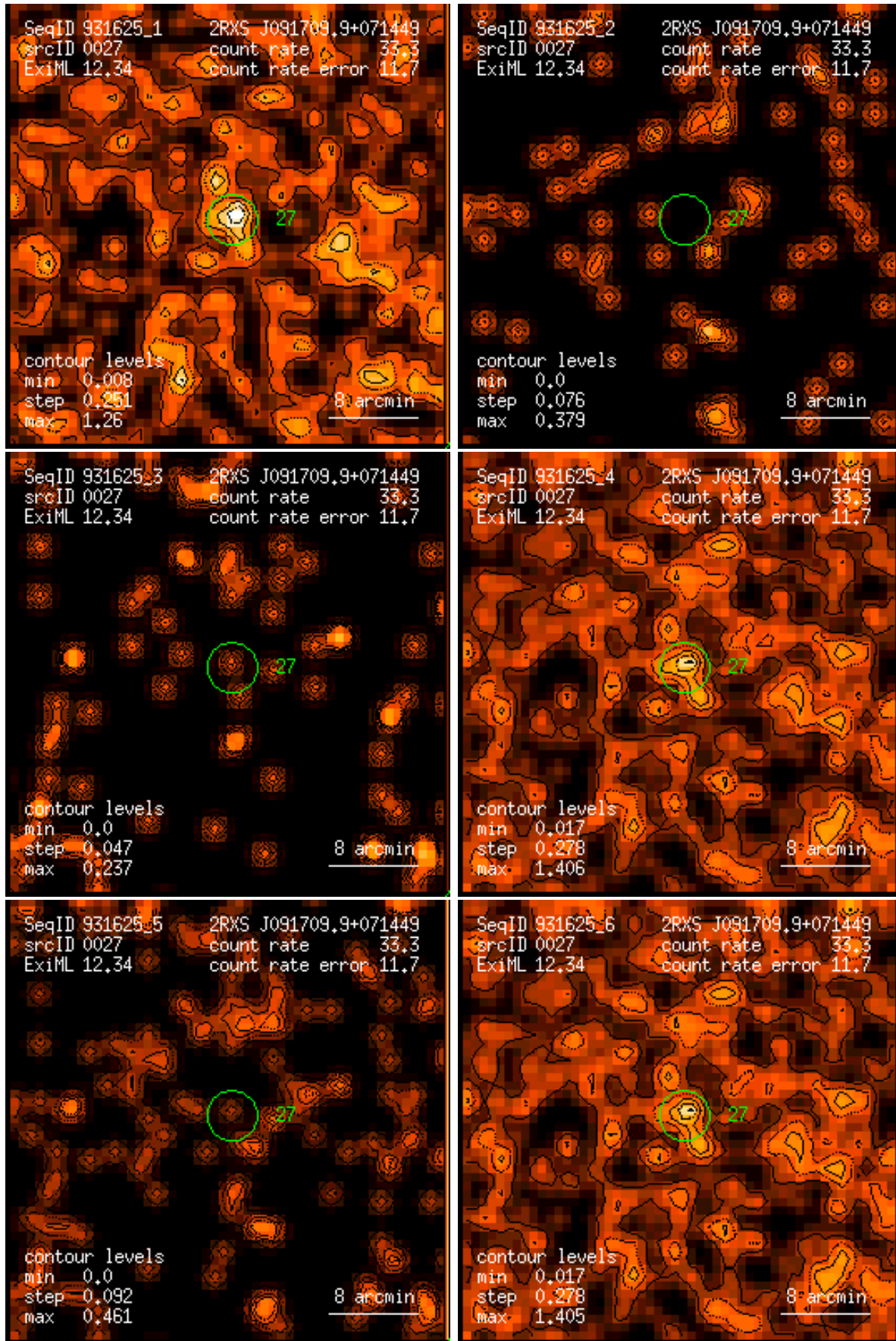
Figure 27: RASS 931625: detection 0027: band rate images, Gaussian filter: (1) PSPC channels 11 – 41, (2) 52 – 90, (3) 91 – 201, (4) 11 – 235, (5) 52 – 201, (6) 11 – 201. Broad band rates in counts/ks. Band rate contour levels in counts/ks/arcmin 2 .
