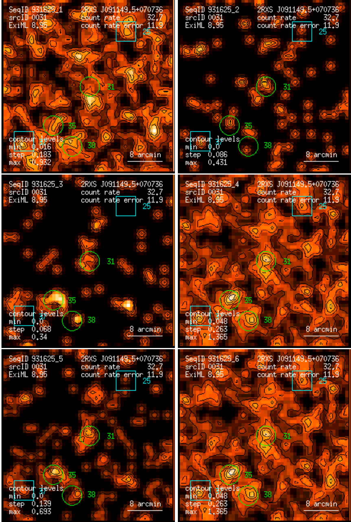
Figure 31: RASS 931625: detection 0031: band rate images, Gaussian filter: (1) PSPC channels 11 – 41, (2) 52 – 90, (3) 91 – 201, (4) 11 – 235, (5) 52 – 201, (6) 11 – 201. Broad band rates in counts/ks. Band rate contour levels in counts/ks/arcmin 2 .
