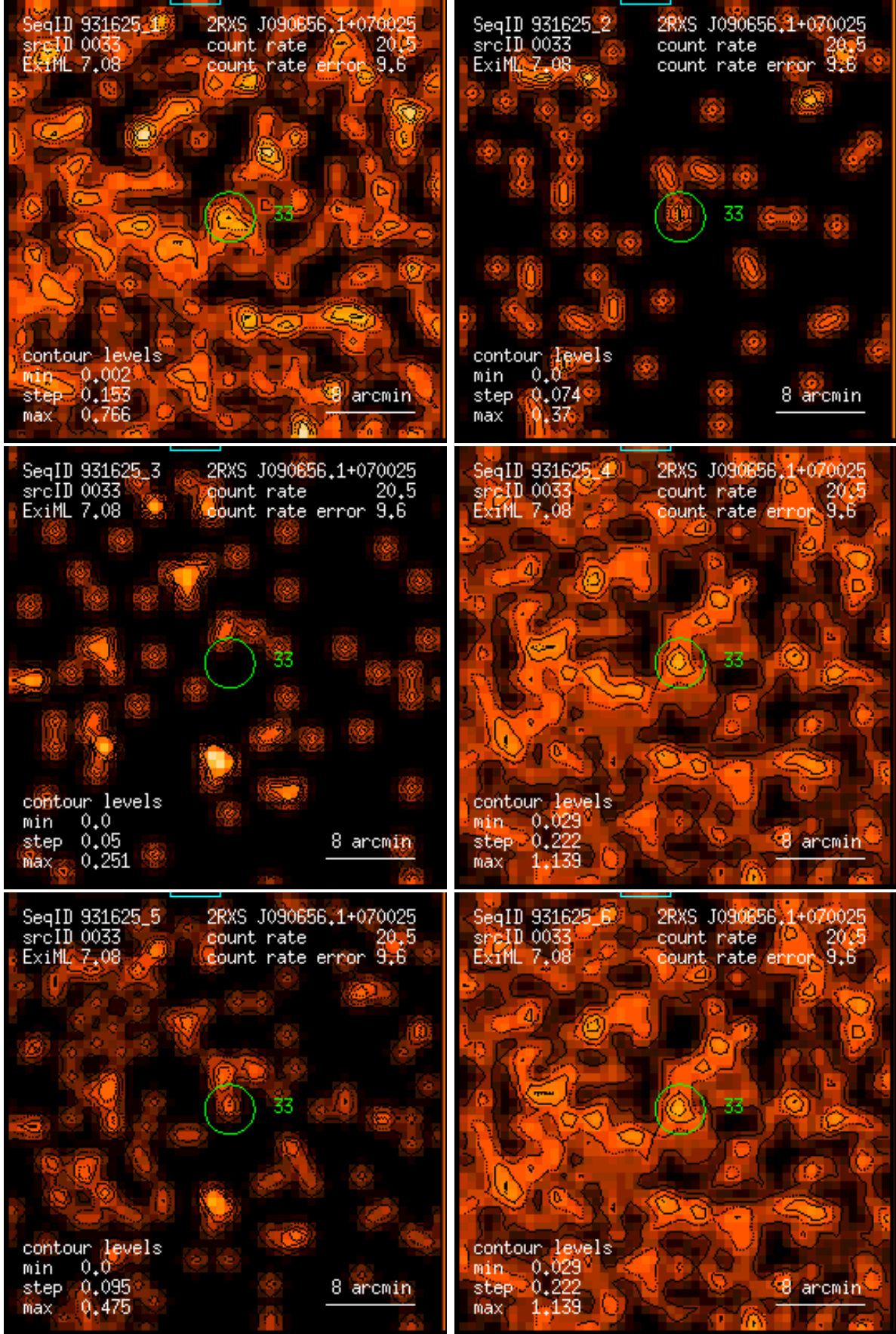
Figure 33: RASS 931625: detection 0033: band rate images, Gaussian filter: (1) PSPC channels 11 – 41, (2) 52 – 90, (3) 91 – 201, (4) 11 – 235, (5) 52 – 201, (6) 11 – 201. Broad band rates in counts/ks. Band rate contour levels in counts/ks/arcmin 2 .
