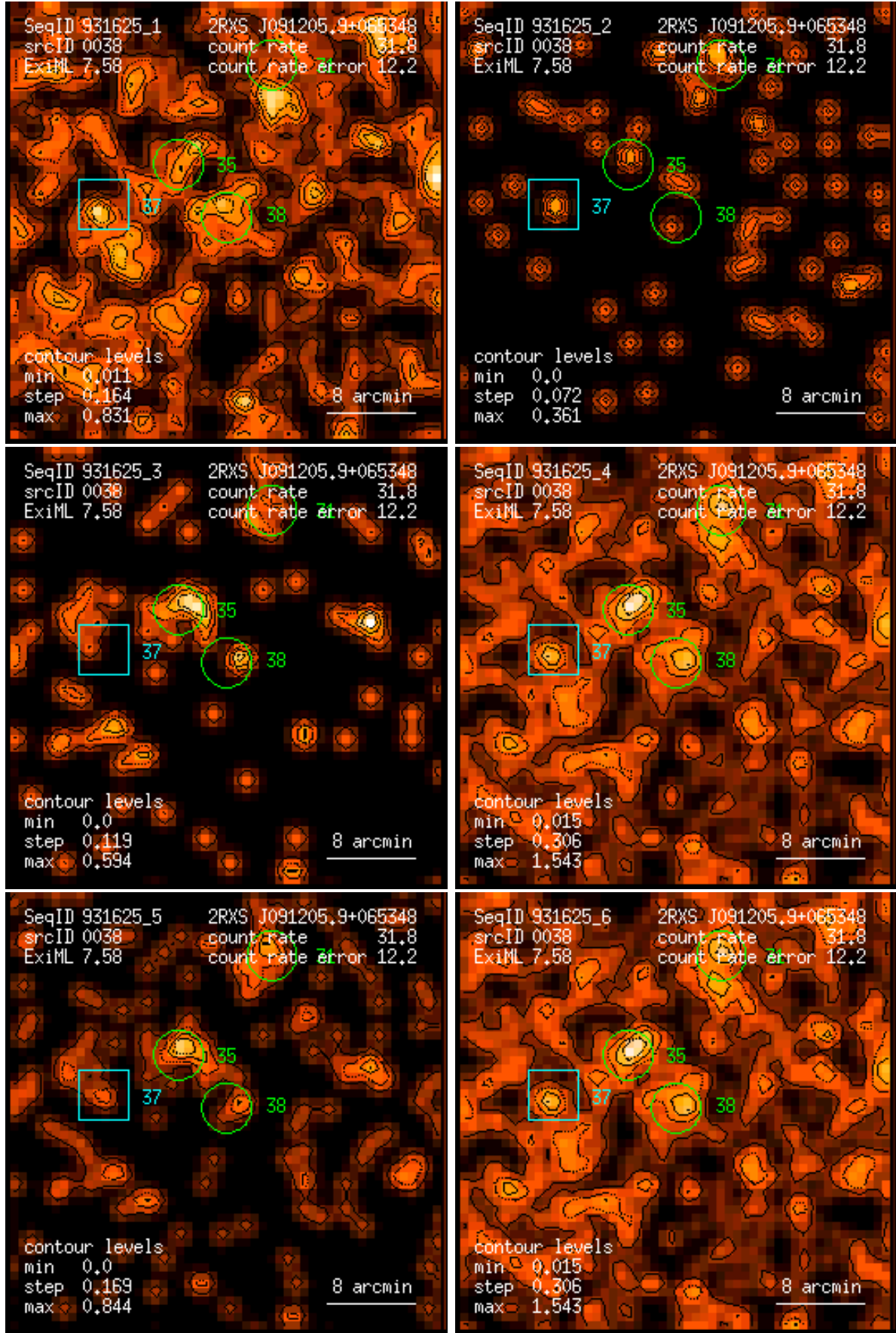
Figure 38: RASS 931625: detection 0038: band rate images, Gaussian filter: (1) PSPC channels 11 – 41, (2) 52 – 90, (3) 91 – 201, (4) 11 – 235, (5) 52 – 201, (6) 11 – 201. Broad band rates in counts/ks. Band rate contour levels in counts/ks/arcmin 2 .
