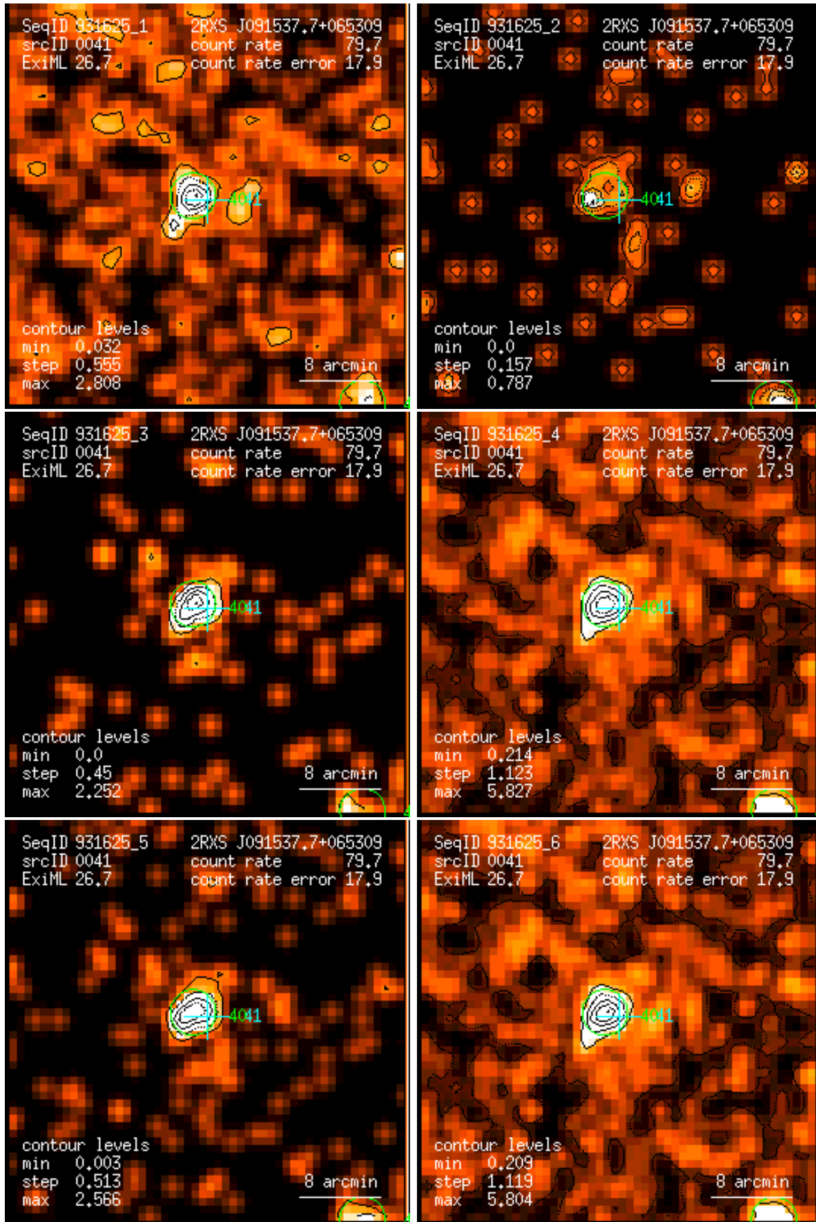
Figure 41: RASS 931625: detection 0041: band rate images, Gaussian filter: (1) PSPC channels 11 – 41, (2) 52 – 90, (3) 91 – 201, (4) 11 – 235, (5) 52 – 201, (6) 11 – 201. Broad band rates in counts/ks. Band rate contour levels in counts/ks/arcmin 2 .
