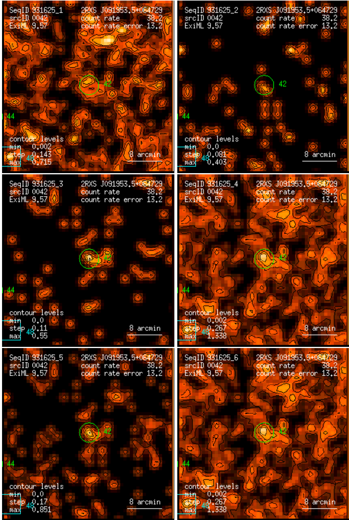
Figure 42: RASS 931625: detection 0042: band rate images, Gaussian filter: (1) PSPC channels 11 – 41, (2) 52 – 90, (3) 91 – 201, (4) 11 – 235, (5) 52 – 201, (6) 11 – 201. Broad band rates in counts/ks. Band rate contour levels in counts/ks/arcmin 2 .
