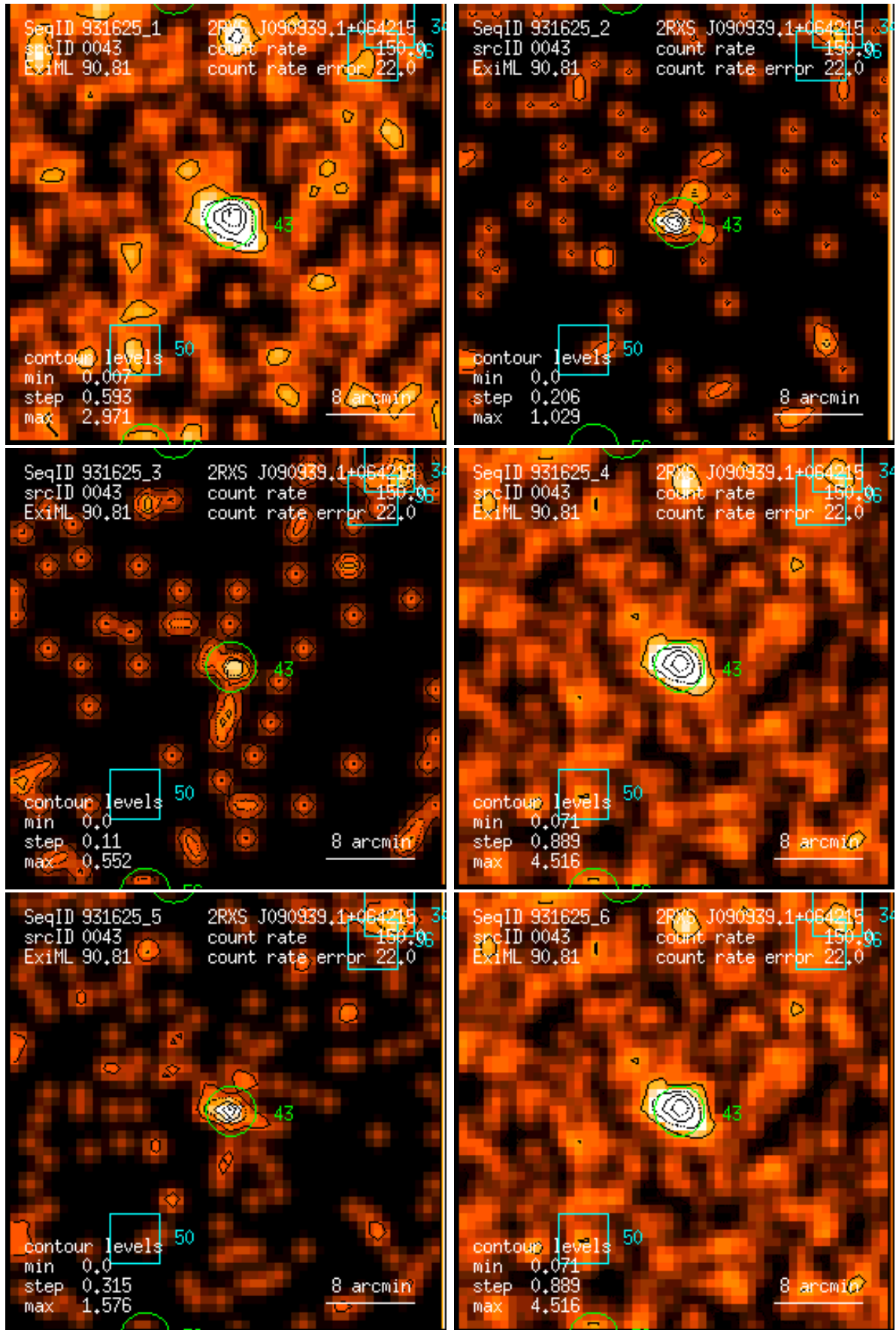
Figure 43: RASS 931625: detection 0043: band rate images, Gaussian filter: (1) PSPC channels 11 – 41, (2) 52 – 90, (3) 91 – 201, (4) 11 – 235, (5) 52 – 201, (6) 11 – 201. Broad band rates in counts/ks. Band rate contour levels in counts/ks/arcmin 2 .
