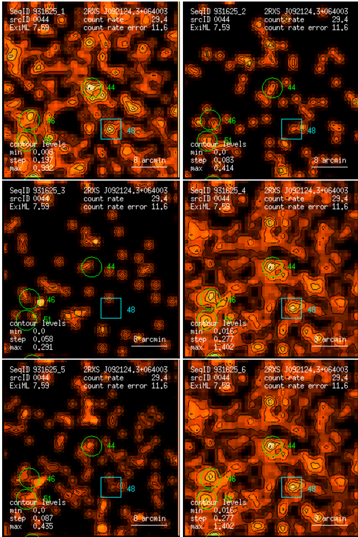
Figure 44: RASS 931625: detection 0044: band rate images, Gaussian filter: (1) PSPC channels 11 – 41, (2) 52 – 90, (3) 91 – 201, (4) 11 – 235, (5) 52 – 201, (6) 11 – 201. Broad band rates in counts/ks. Band rate contour levels in counts/ks/arcmin 2 .
