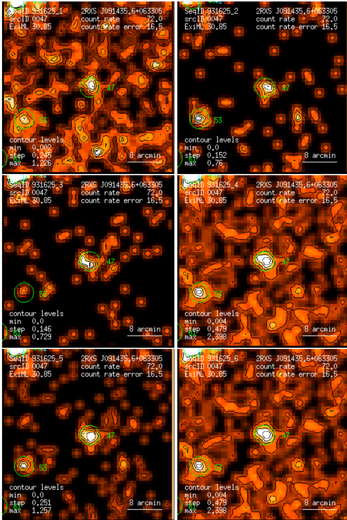
Figure 47: RASS 931625: detection 0047: band rate images, Gaussian filter: (1) PSPC channels 11 – 41, (2) 52 – 90, (3) 91 – 201, (4) 11 – 235, (5) 52 – 201, (6) 11 – 201. Broad band rates in counts/ks. Band rate contour levels in counts/ks/arcmin 2 .
