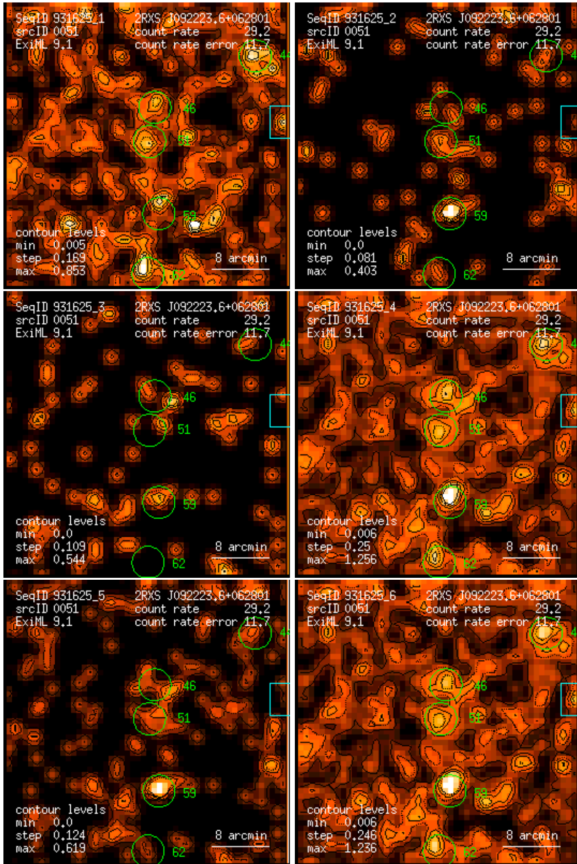
Figure 51: RASS 931625: detection 0051: band rate images, Gaussian filter: (1) PSPC channels 11 – 41, (2) 52 – 90, (3) 91 – 201, (4) 11 – 235, (5) 52 – 201, (6) 11 – 201. Broad band rates in counts/ks. Band rate contour levels in counts/ks/arcmin 2 .
