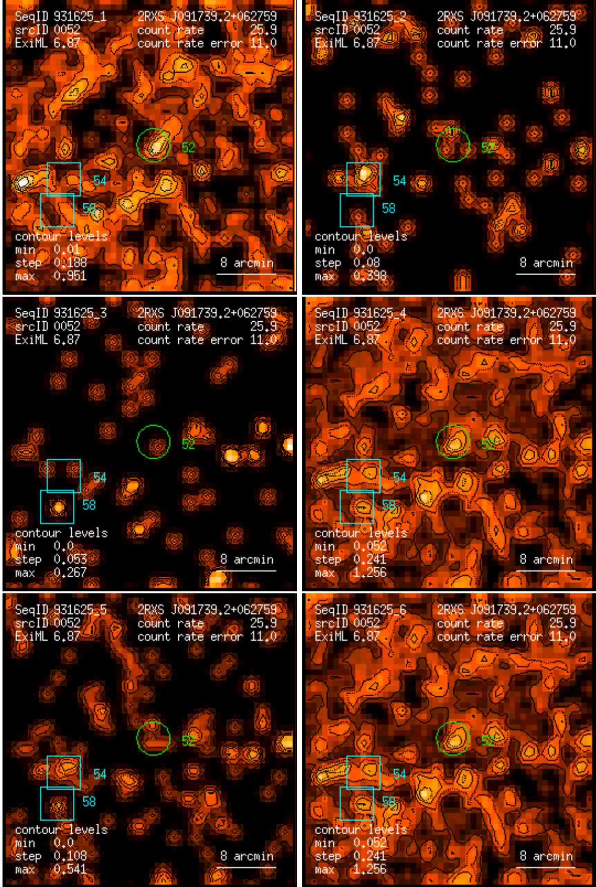
Figure 52: RASS 931625: detection 0052: band rate images, Gaussian filter: (1) PSPC channels 11 – 41, (2) 52 – 90, (3) 91 – 201, (4) 11 – 235, (5) 52 – 201, (6) 11 – 201. Broad band rates in counts/ks. Band rate contour levels in counts/ks/arcmin 2 .
