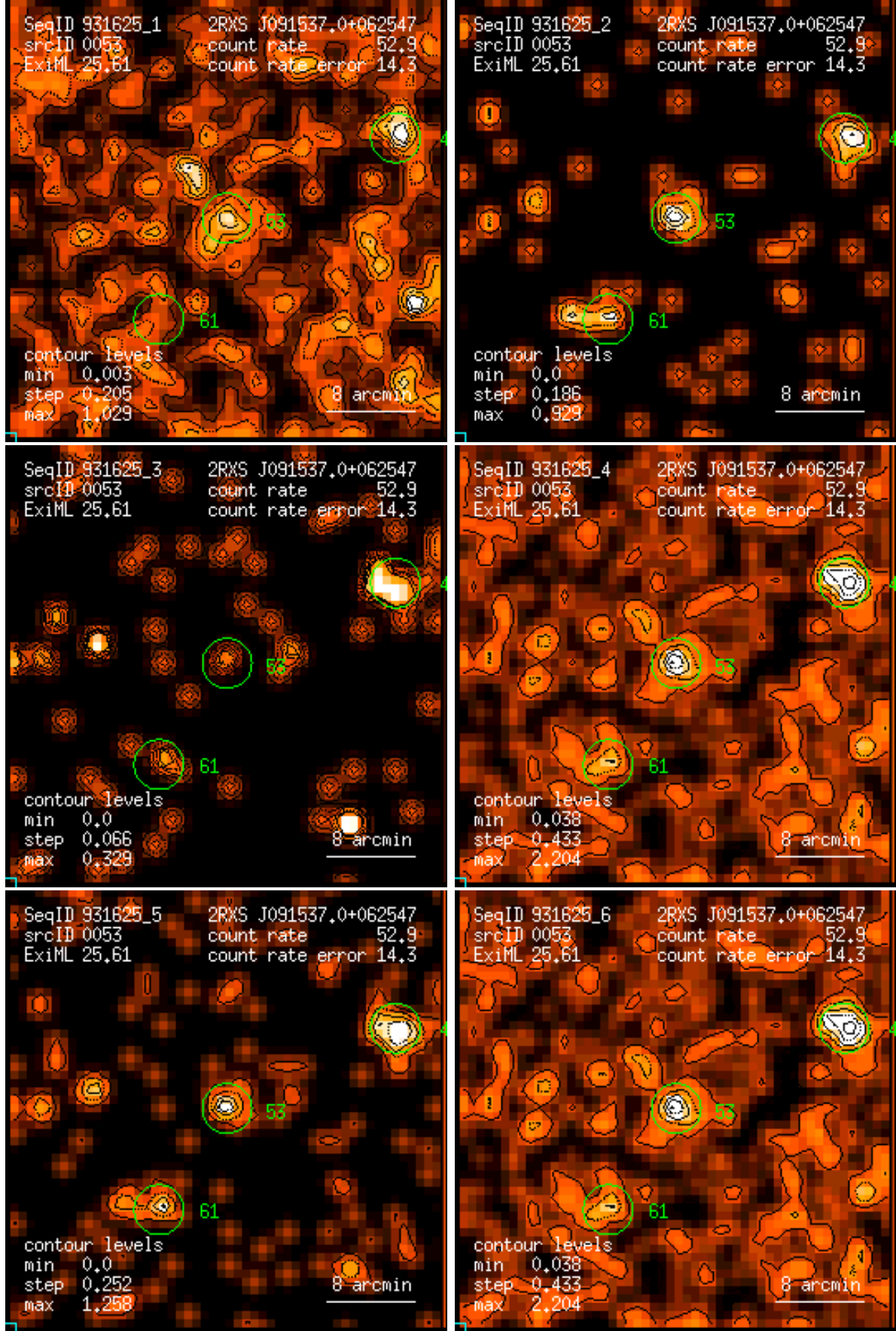
Figure 53: RASS 931625: detection 0053: band rate images, Gaussian filter: (1) PSPC channels 11 – 41, (2) 52 – 90, (3) 91 – 201, (4) 11 – 235, (5) 52 – 201, (6) 11 – 201. Broad band rates in counts/ks. Band rate contour levels in counts/ks/arcmin 2 .
