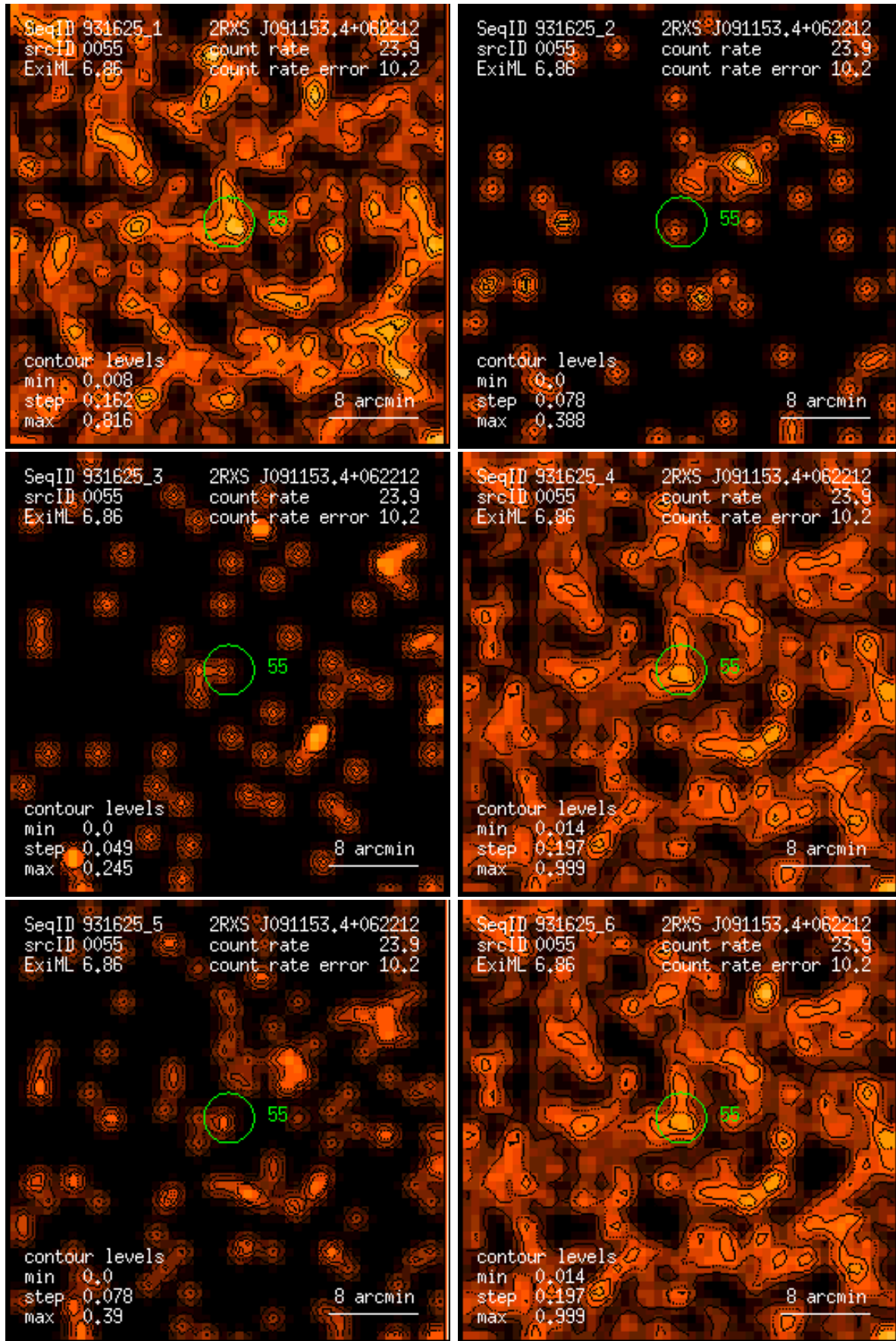
Figure 55: RASS 931625: detection 0055: band rate images, Gaussian filter: (1) PSPC channels 11 – 41, (2) 52 – 90, (3) 91 – 201, (4) 11 – 235, (5) 52 – 201, (6) 11 – 201. Broad band rates in counts/ks. Band rate contour levels in counts/ks/arcmin 2 .
