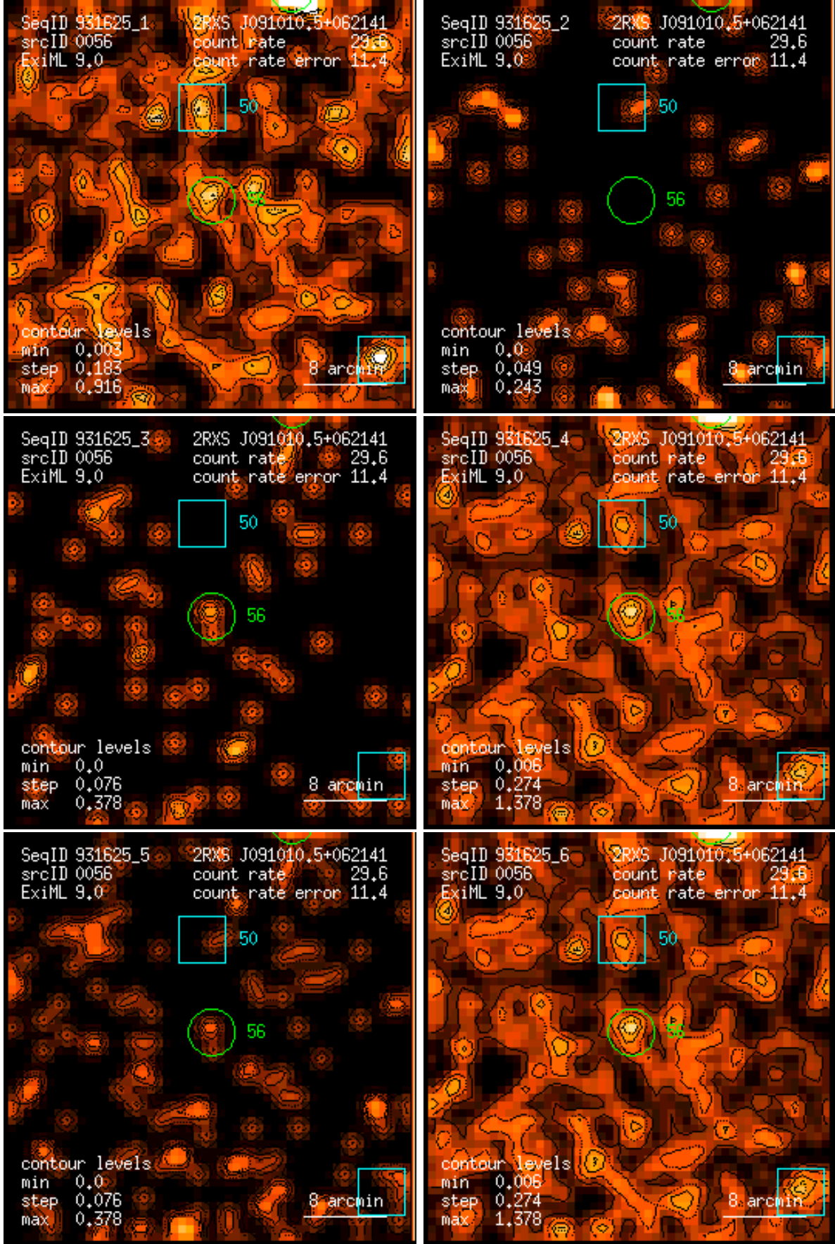
Figure 56: RASS 931625: detection 0056: band rate images, Gaussian filter: (1) PSPC channels 11 – 41, (2) 52 – 90, (3) 91 – 201, (4) 11 – 235, (5) 52 – 201, (6) 11 – 201. Broad band rates in counts/ks. Band rate contour levels in counts/ks/arcmin 2 .
