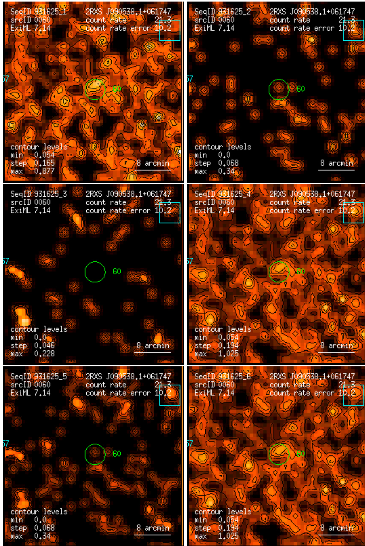
Figure 60: RASS 931625: detection 0060: band rate images, Gaussian filter: (1) PSPC channels 11 – 41, (2) 52 – 90, (3) 91 – 201, (4) 11 – 235, (5) 52 – 201, (6) 11 – 201. Broad band rates in counts/ks. Band rate contour levels in counts/ks/arcmin 2 .
