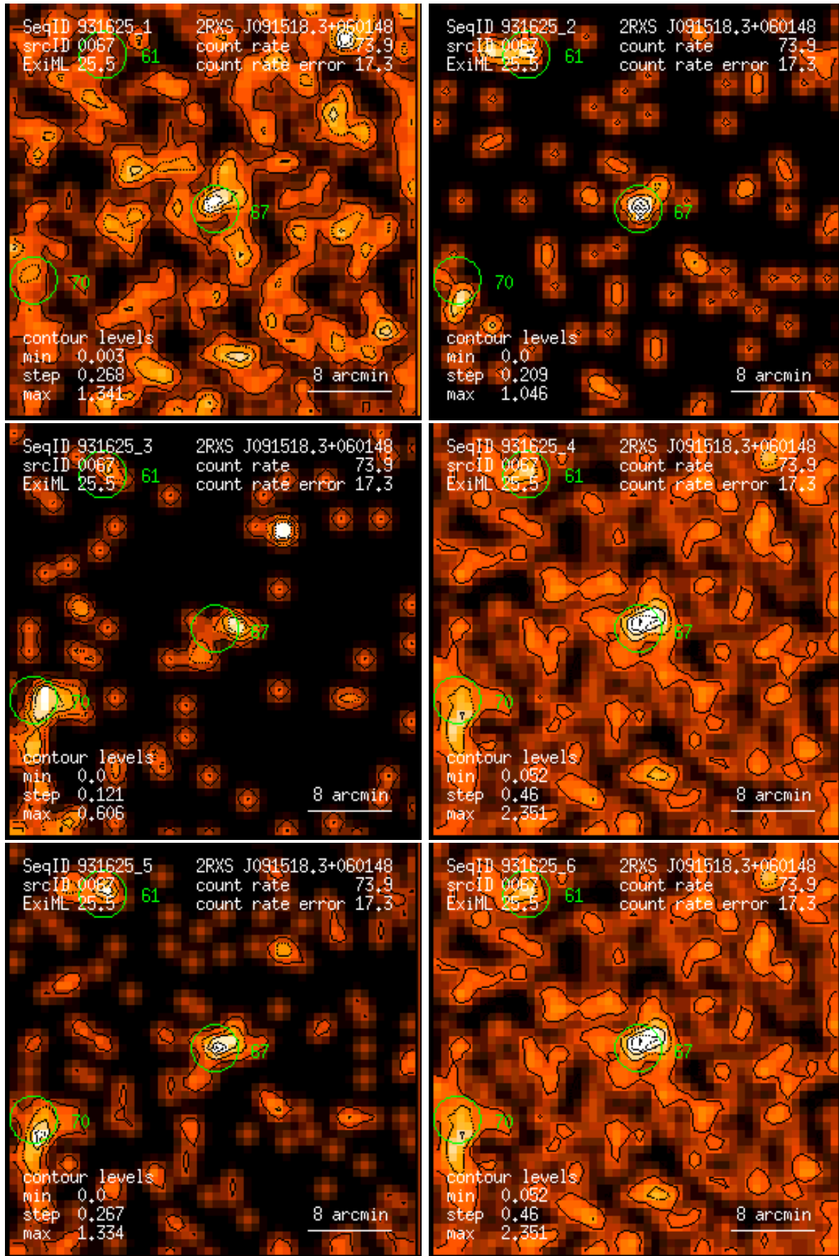
Figure 67: RASS 931625: detection 0067: band rate images, Gaussian filter: (1) PSPC channels 11 – 41, (2) 52 – 90, (3) 91 – 201, (4) 11 – 235, (5) 52 – 201, (6) 11 – 201. Broad band rates in counts/ks. Band rate contour levels in counts/ks/arcmin 2 .
