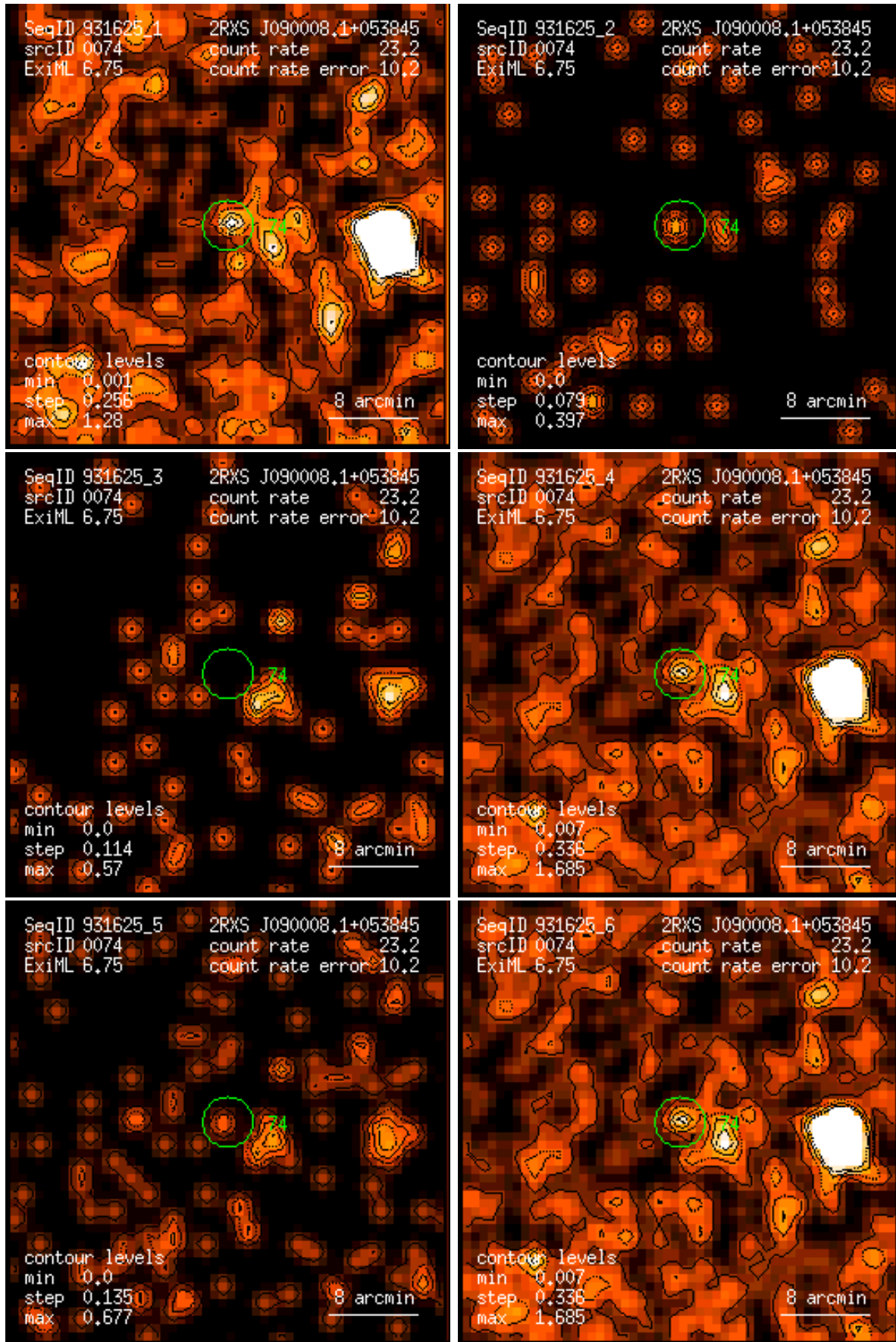
Figure 74: RASS 931625: detection 0074: band rate images, Gaussian filter: (1) PSPC channels 11 – 41, (2) 52 – 90, (3) 91 – 201, (4) 11 – 235, (5) 52 – 201, (6) 11 – 201. Broad band rates in counts/ks. Band rate contour levels in counts/ks/arcmin 2 .
