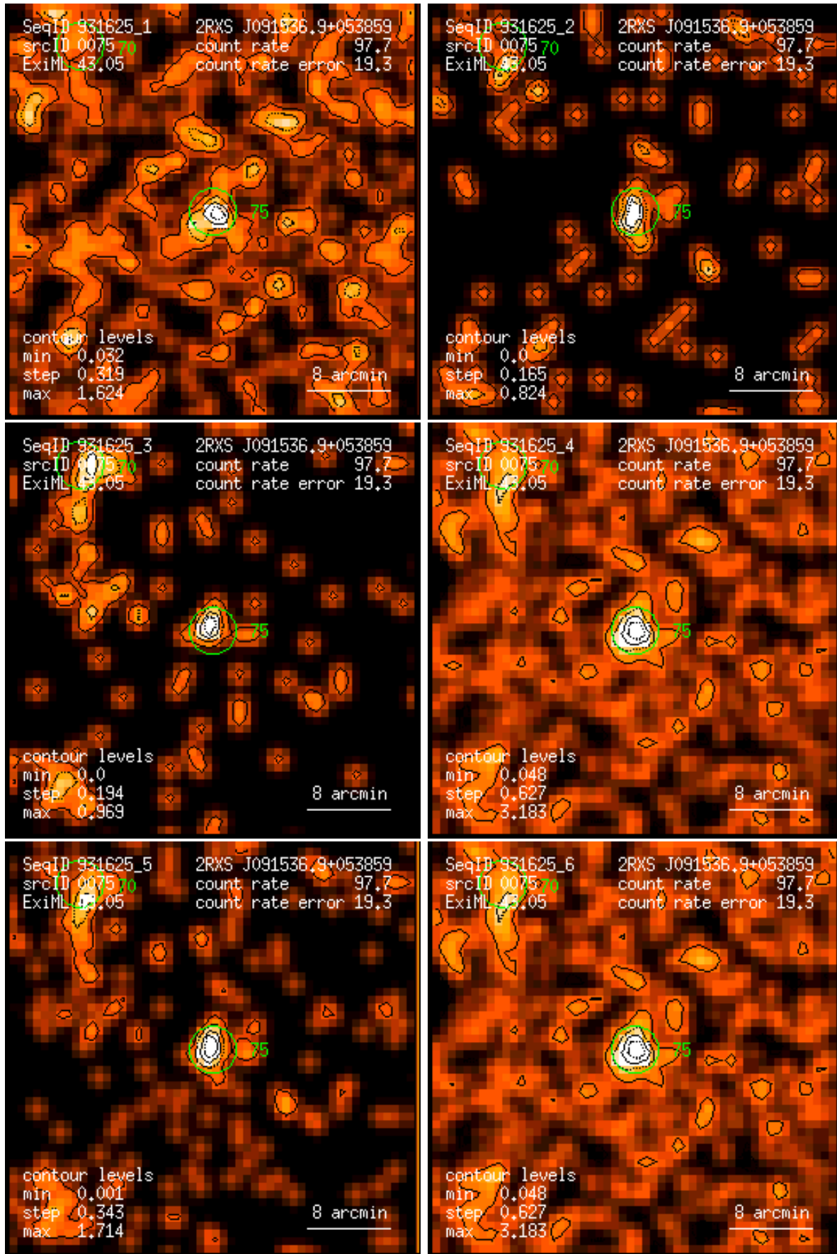
Figure 75: RASS 931625: detection 0075: band rate images, Gaussian filter: (1) PSPC channels 11 – 41, (2) 52 – 90, (3) 91 – 201, (4) 11 – 235, (5) 52 – 201, (6) 11 – 201. Broad band rates in counts/ks. Band rate contour levels in counts/ks/arcmin 2 .
