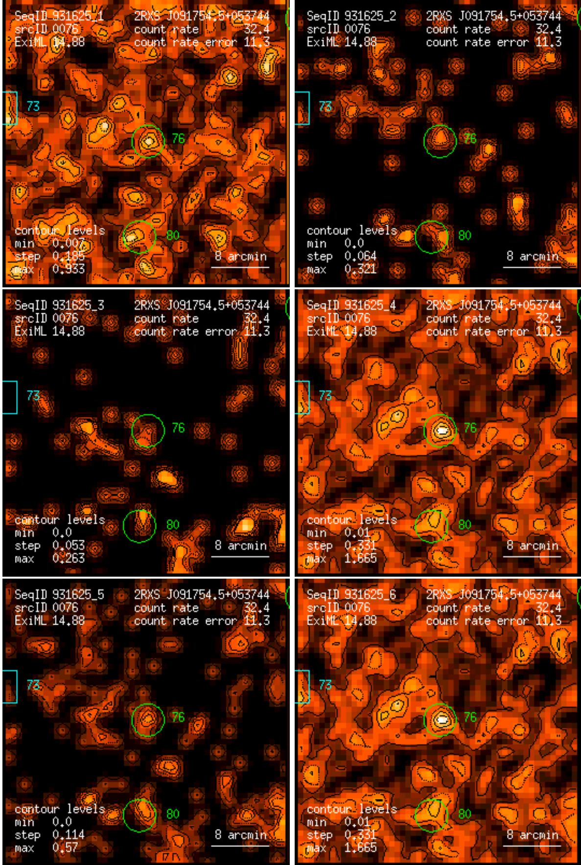
Figure 76: RASS 931625: detection 0076: band rate images, Gaussian filter: (1) PSPC channels 11 – 41, (2) 52 – 90, (3) 91 – 201, (4) 11 – 235, (5) 52 – 201, (6) 11 – 201. Broad band rates in counts/ks. Band rate contour levels in counts/ks/arcmin 2 .
