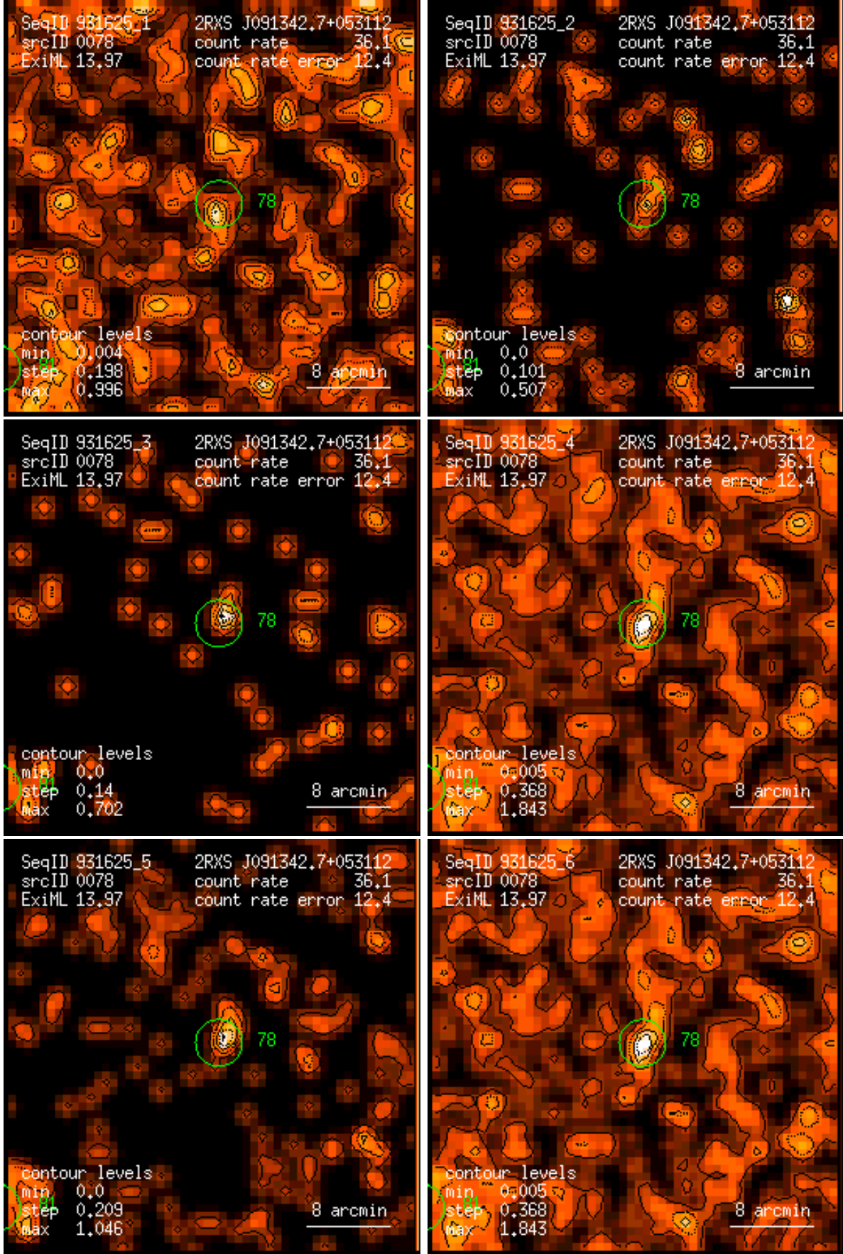
Figure 78: RASS 931625: detection 0078: band rate images, Gaussian filter: (1) PSPC channels 11 – 41, (2) 52 – 90, (3) 91 – 201, (4) 11 – 235, (5) 52 – 201, (6) 11 – 201. Broad band rates in counts/ks. Band rate contour levels in counts/ks/arcmin 2 .
