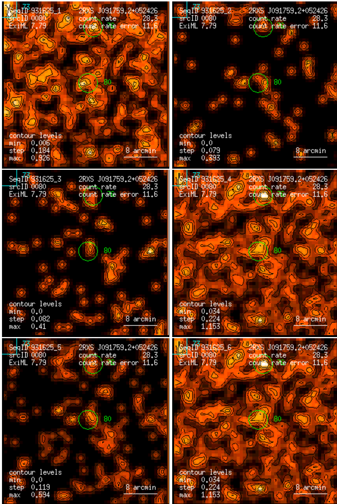
Figure 80: RASS 931625: detection 0080: band rate images, Gaussian filter: (1) PSPC channels 11 – 41, (2) 52 – 90, (3) 91 – 201, (4) 11 – 235, (5) 52 – 201, (6) 11 – 201. Broad band rates in counts/ks. Band rate contour levels in counts/ks/arcmin 2 .
