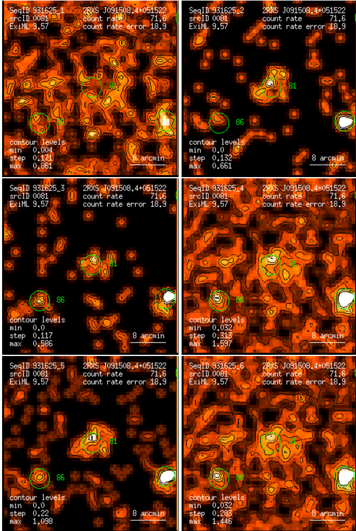
Figure 81: RASS 931625: detection 0081: band rate images, Gaussian filter: (1) PSPC channels 11 – 41, (2) 52 – 90, (3) 91 – 201, (4) 11 – 235, (5) 52 – 201, (6) 11 – 201. Broad band rates in counts/ks. Band rate contour levels in counts/ks/arcmin 2 .
