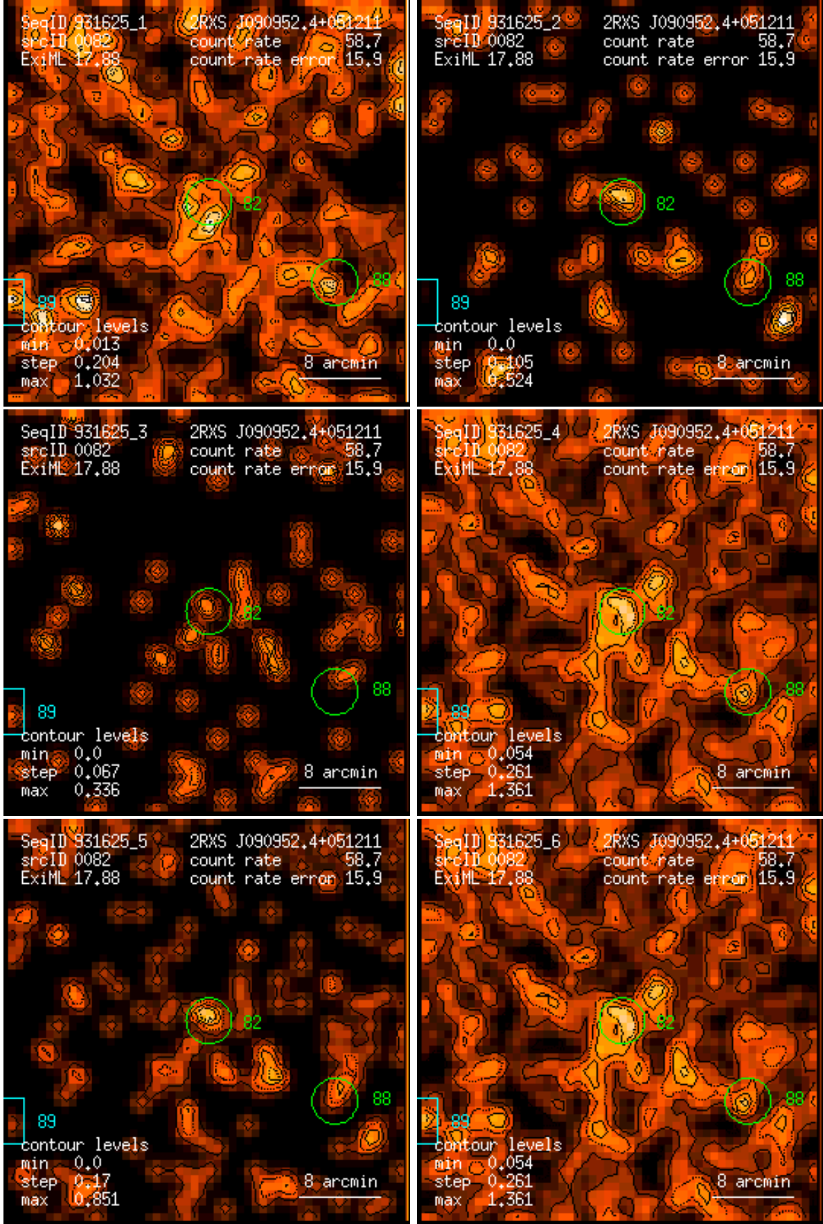
Figure 82: RASS 931625: detection 0082: band rate images, Gaussian filter: (1) PSPC channels 11 – 41, (2) 52 – 90, (3) 91 – 201, (4) 11 – 235, (5) 52 – 201, (6) 11 – 201. Broad band rates in counts/ks. Band rate contour levels in counts/ks/arcmin 2 .
