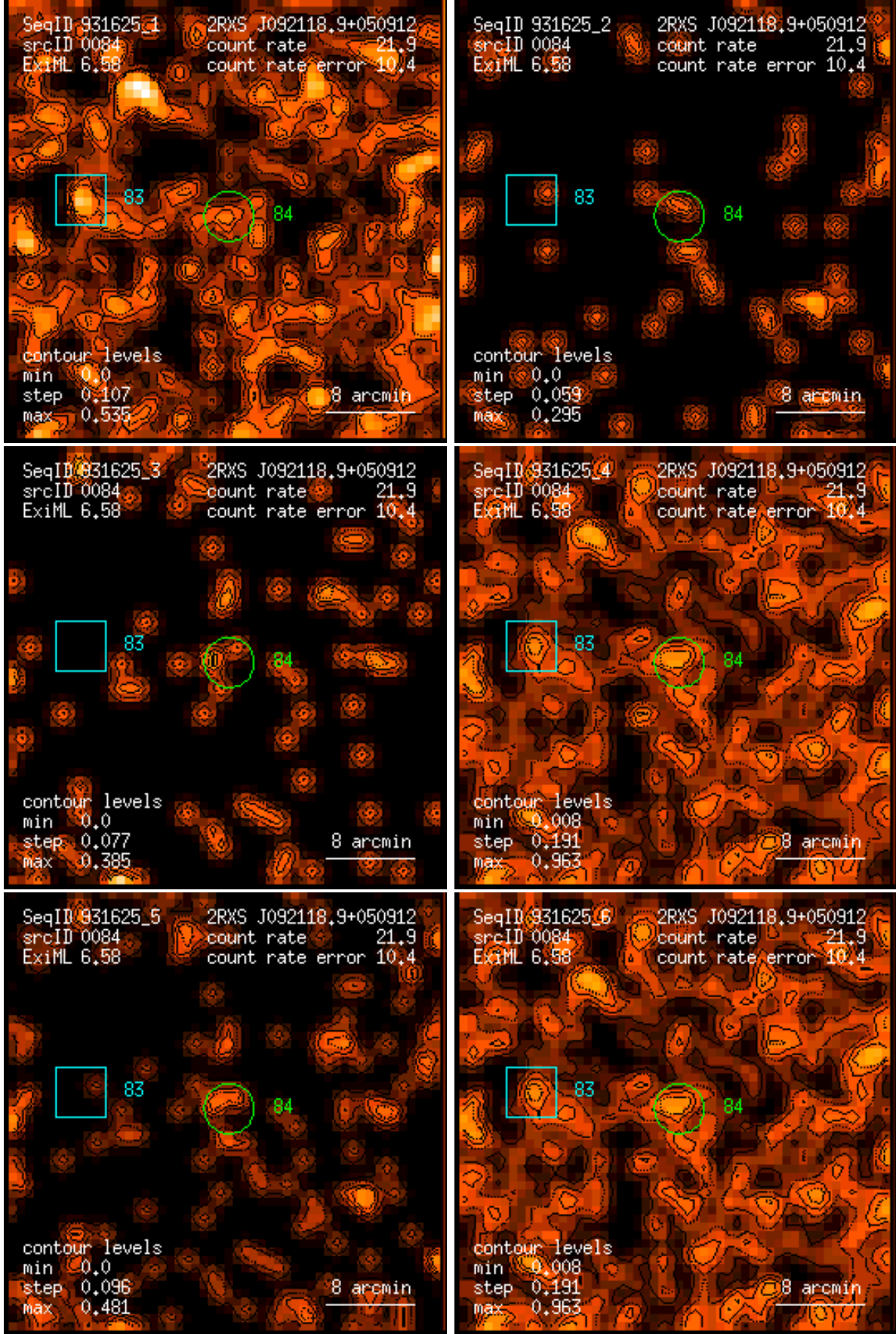
Figure 84: RASS 931625: detection 0084: band rate images, Gaussian filter: (1) PSPC channels 11 – 41, (2) 52 – 90, (3) 91 – 201, (4) 11 – 235, (5) 52 – 201, (6) 11 – 201. Broad band rates in counts/ks. Band rate contour levels in counts/ks/arcmin 2 .
