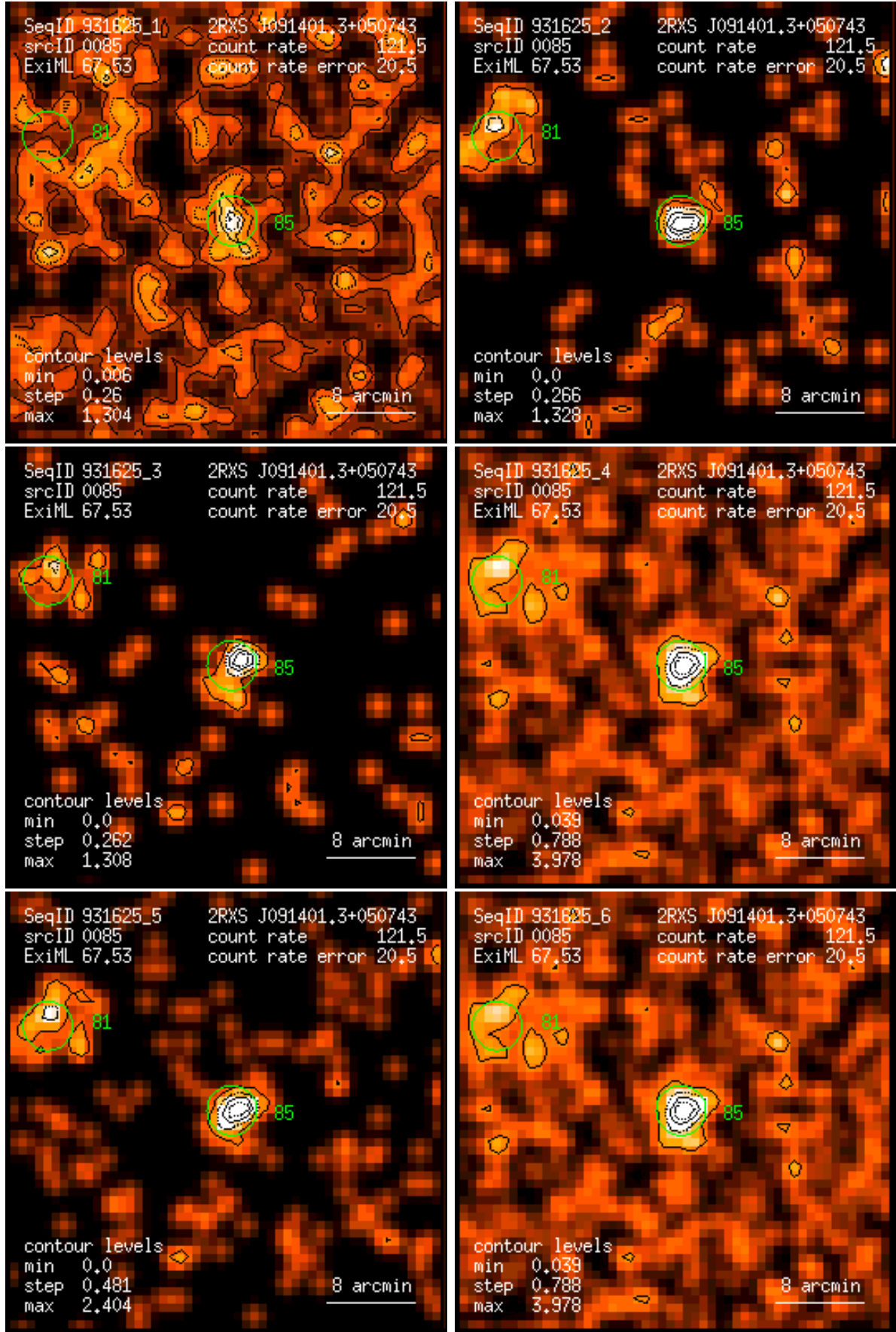
Figure 85: RASS 931625: detection 0085: band rate images, Gaussian filter: (1) PSPC channels 11 – 41, (2) 52 – 90, (3) 91 – 201, (4) 11 – 235, (5) 52 – 201, (6) 11 – 201. Broad band rates in counts/ks. Band rate contour levels in counts/ks/arcmin 2 .
