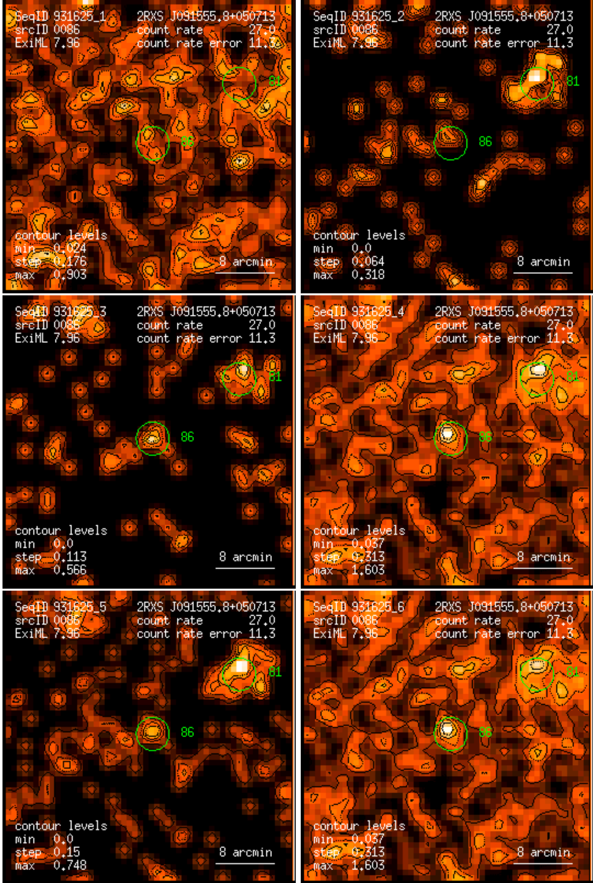
Figure 86: RASS 931625: detection 0086: band rate images, Gaussian filter: (1) PSPC channels 11 – 41, (2) 52 – 90, (3) 91 – 201, (4) 11 – 235, (5) 52 – 201, (6) 11 – 201. Broad band rates in counts/ks. Band rate contour levels in counts/ks/arcmin 2 .
