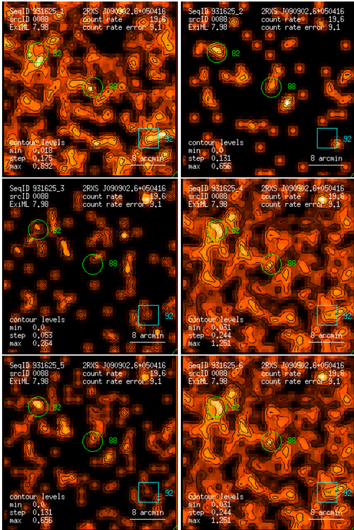
Figure 88: RASS 931625: detection 0088: band rate images, Gaussian filter: (1) PSPC channels 11 – 41, (2) 52 – 90, (3) 91 – 201, (4) 11 – 235, (5) 52 – 201, (6) 11 – 201. Broad band rates in counts/ks. Band rate contour levels in counts/ks/arcmin 2 .
