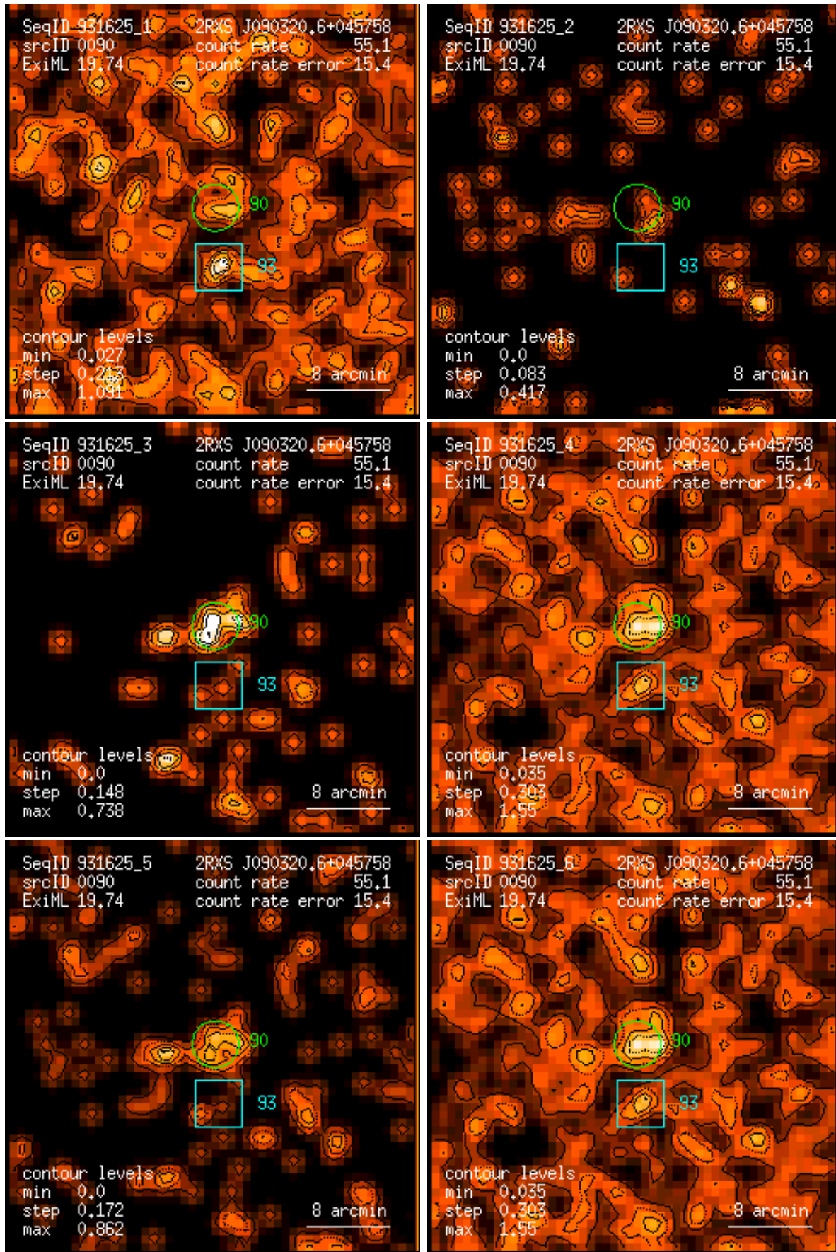
Figure 90: RASS 931625: detection 0090: band rate images, Gaussian filter: (1) PSPC channels 11 – 41, (2) 52 – 90, (3) 91 – 201, (4) 11 – 235, (5) 52 – 201, (6) 11 – 201. Broad band rates in counts/ks. Band rate contour levels in counts/ks/arcmin 2 .
